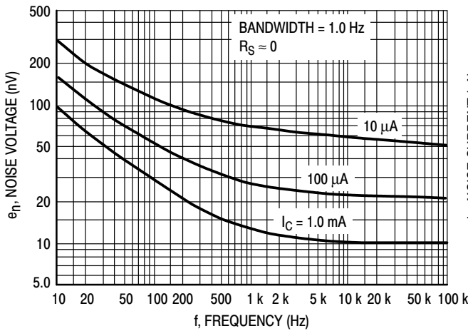
Figure 2. Noise Voltage
