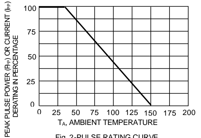
Fig. 2-PULSE RATING CURVE
