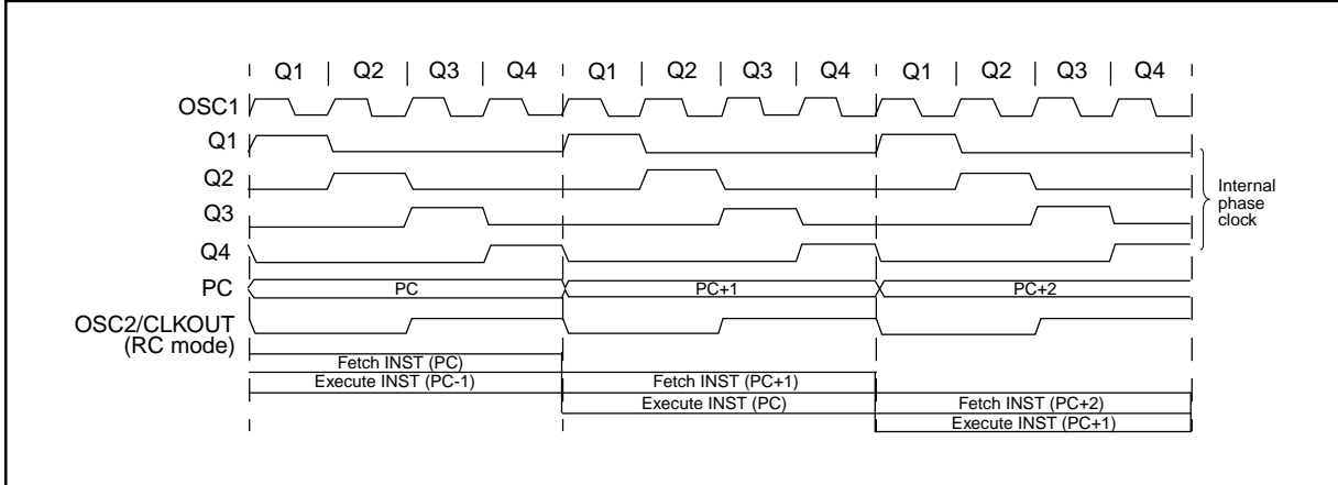
FIGURE 3-2: CLOCK/INSTRUCTION CYCLE
