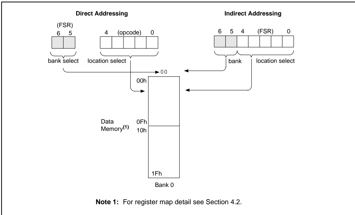
FIGURE 4-6: DIRECT/INDIRECT ADDRESSING
