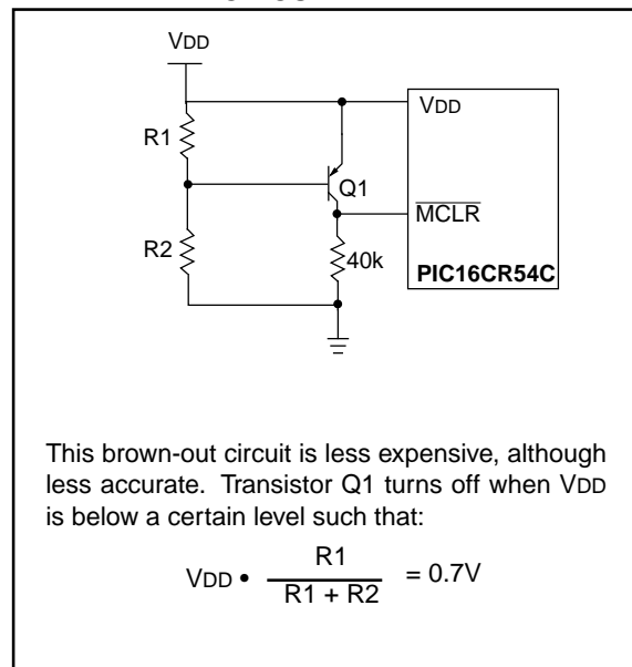
FIGURE 7-14: BROWN-OUT PROTECTION CIRCUIT 2
