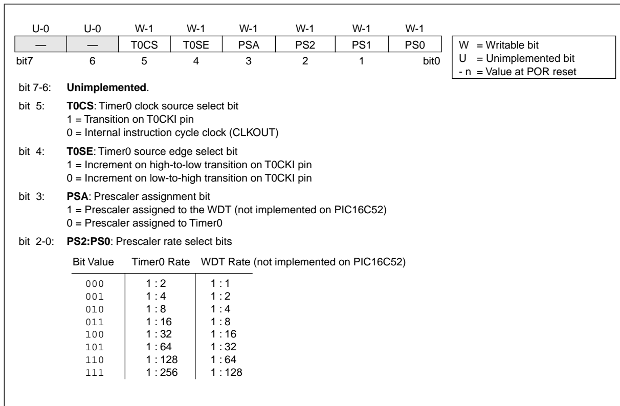
FIGURE 4-4: OPTION REGISTER
