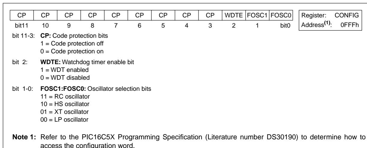
FIGURE 7-1: CONFIGURATION WORD FOR PIC16CR54C
