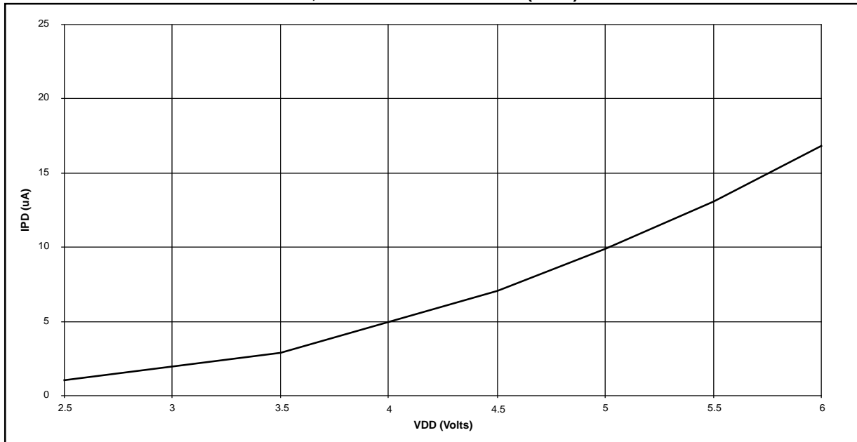
FIGURE 11-6: TYPICAL IPD vs. VDD, WATCHDOG ENABLED (25°C)
