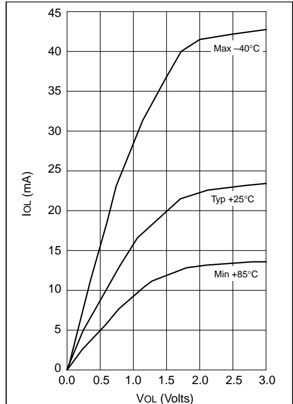
FIGURE 11-18: I_{OL} vs. V_{OL} , V_{DD} = 5\text{ V}
