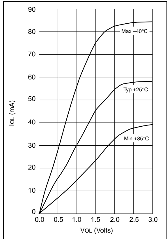
FIGURE 11-18: I_{OL} vs. V_{OL} , V_{DD} = 5\text{ V}
