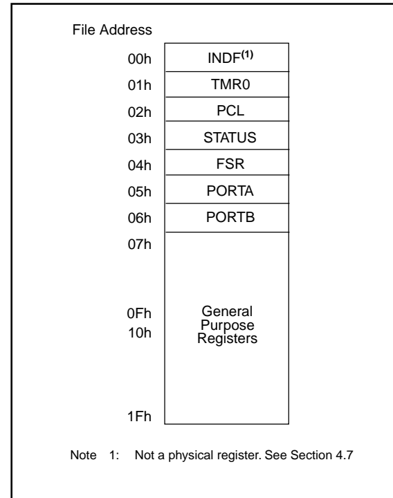
FIGURE 4-2: PIC16CR54C REGISTER FILE MAP
