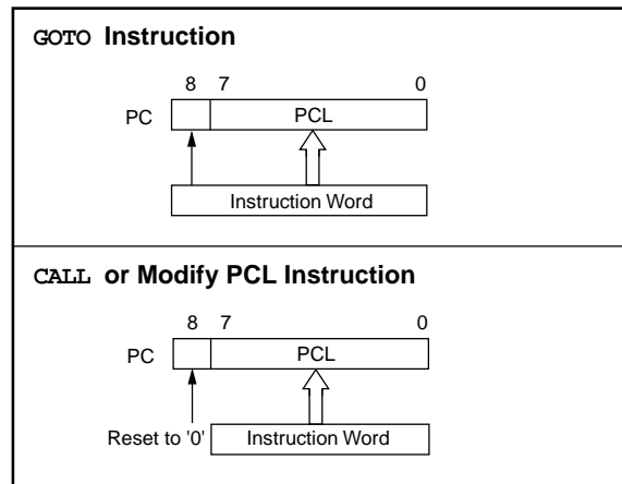
FIGURE 4-5: LOADING OF PC BRANCH INSTRUCTIONS - PIC16CR54C
