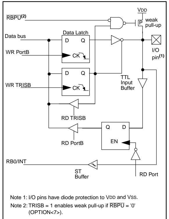
FIGURE 5-6: BLOCK DIAGRAM OF RB3:RB0 PINS
