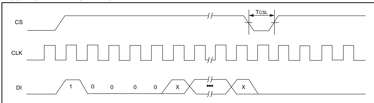
FIGURE 3-4: EWDS TIMING
