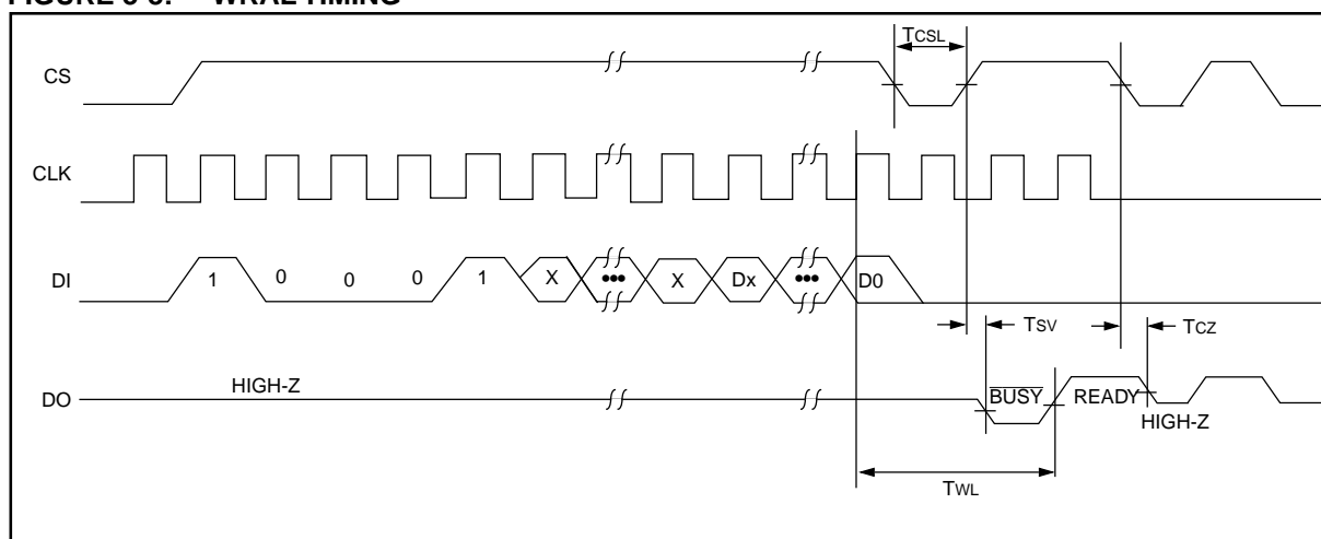
FIGURE 3-8: WRAL TIMING
