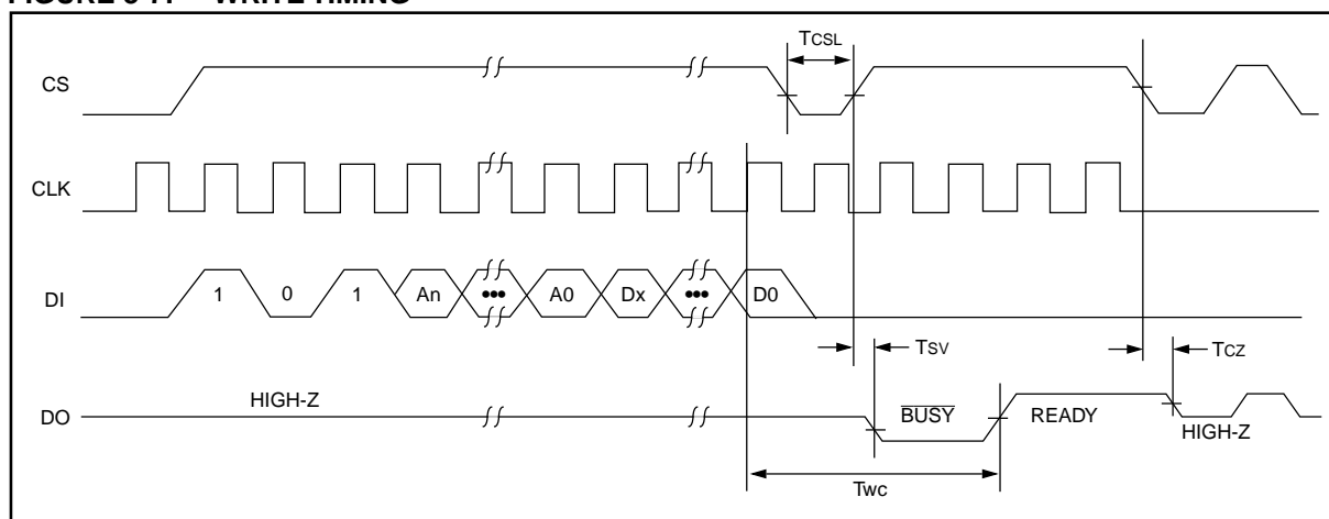
FIGURE 3-7: WRITE TIMING
