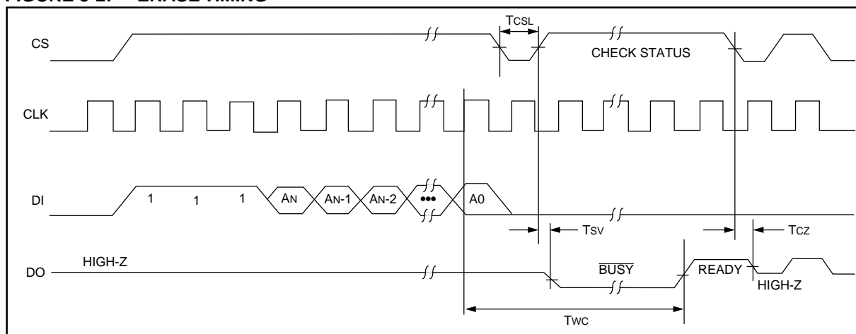
FIGURE 3-2: ERASE TIMING
