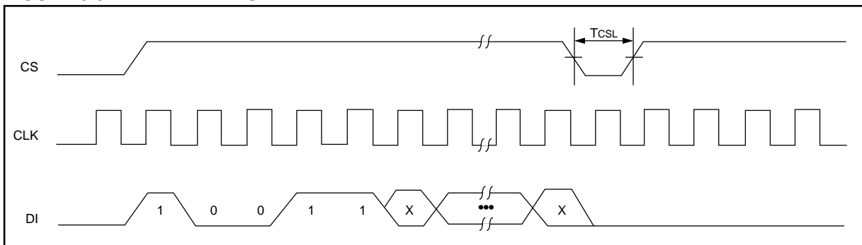
FIGURE 3-6: READ TIMING
