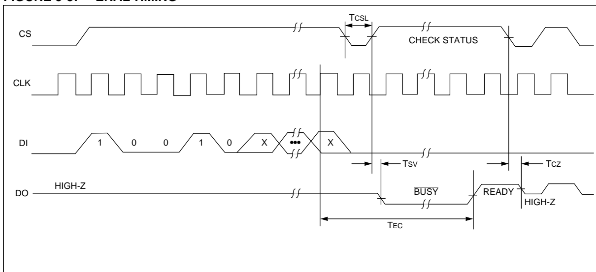
FIGURE 3-3: ERAL TIMING
