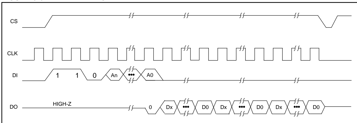
FIGURE 3-6: READ TIMING
