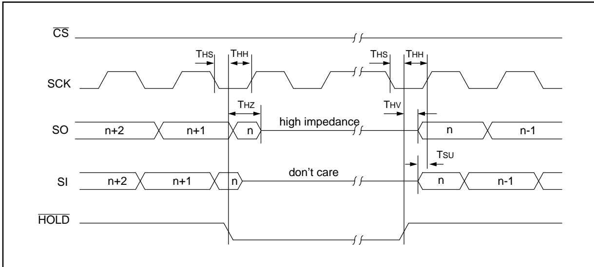
FIGURE 1-2: HOLD TIMING
