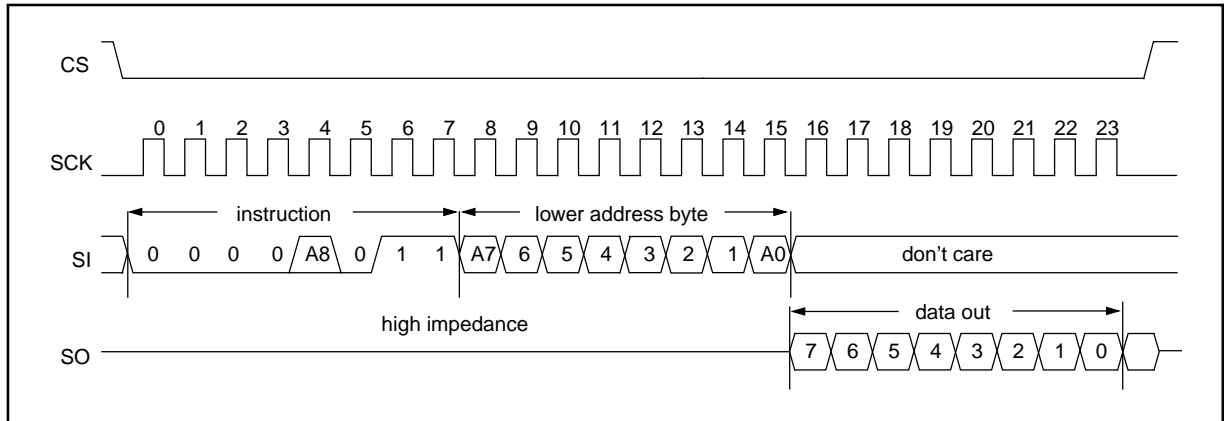
FIGURE 3-1: READ SEQUENCE
