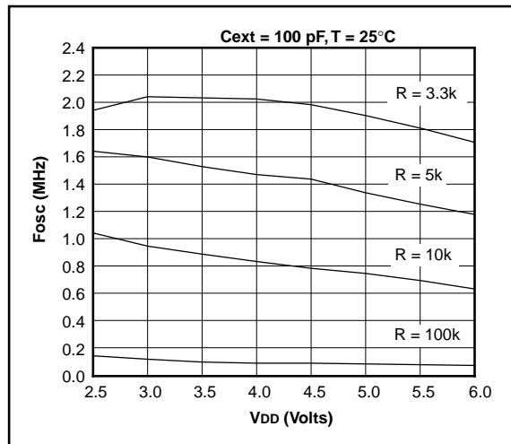
FIGURE 14-6: TYPICAL RC OSCILLATOR FREQUENCY vs. VDD
