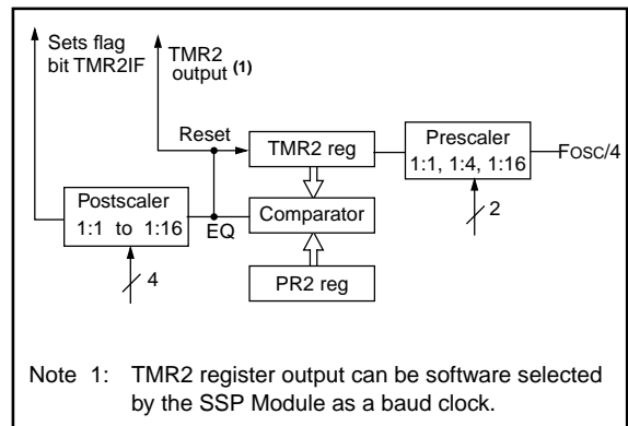
FIGURE 6-1: TIMER2 BLOCK DIAGRAM
