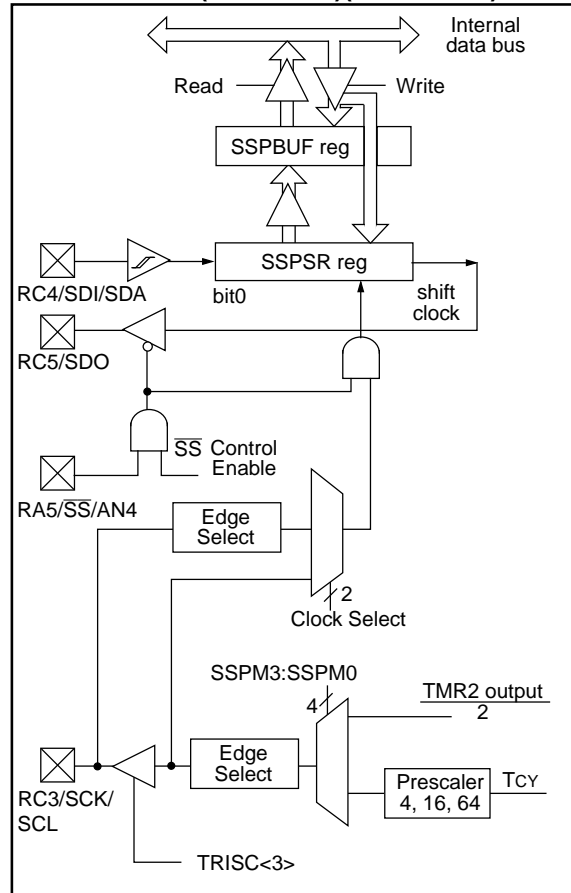
FIGURE 8-6: SSP BLOCK DIAGRAM (SPI MODE)(PIC16C72)
