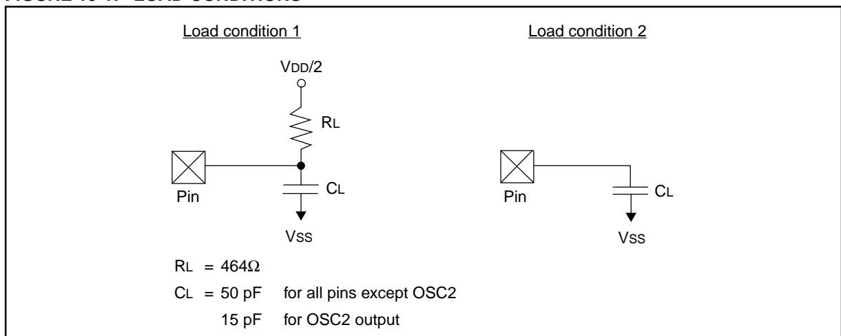
FIGURE 13-1: LOAD CONDITIONS
