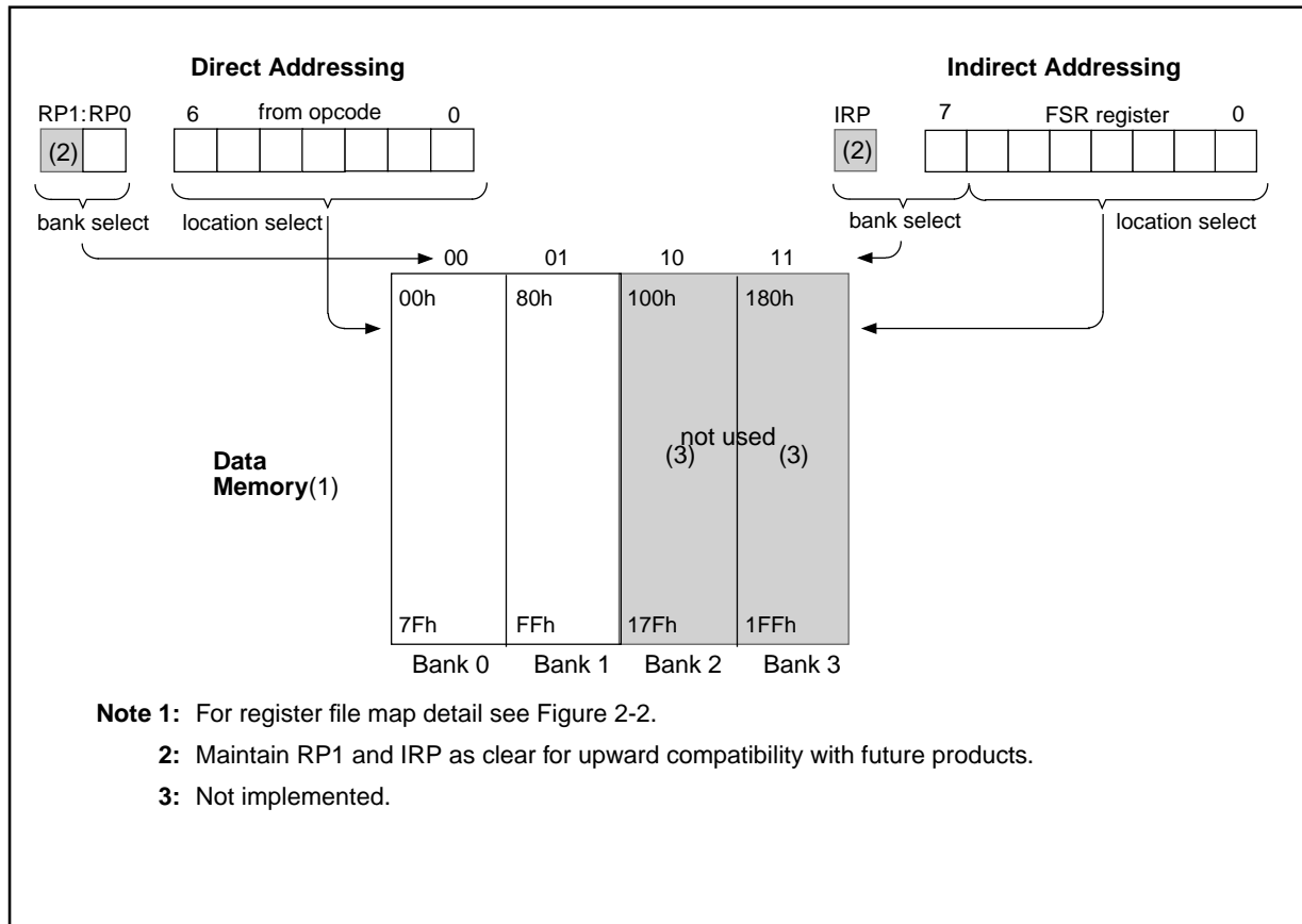
FIGURE 2-11: DIRECT/INDIRECT ADDRESSING
