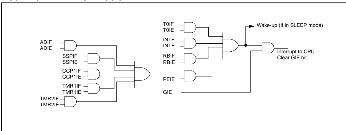
FIGURE 10-11: INTERRUPT LOGIC
