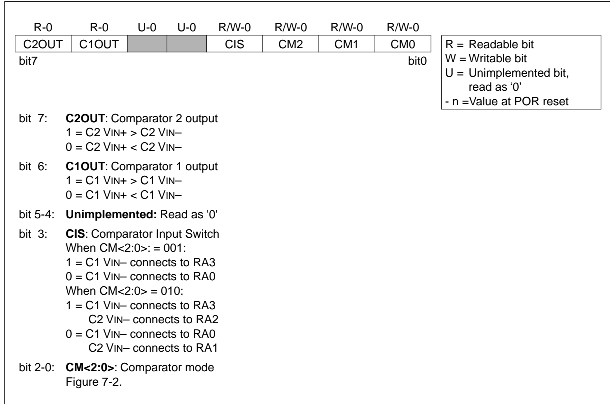
FIGURE 7-1: CMCON REGISTER (ADDRESS 1Fh)
