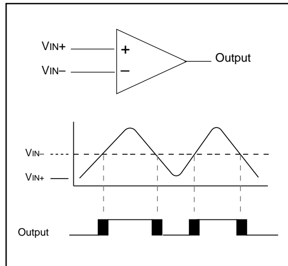
FIGURE 7-3: SINGLE COMPARATOR
