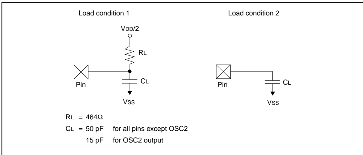
FIGURE 12-7: LOAD CONDITIONS
