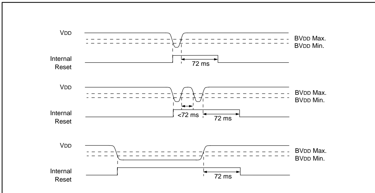
FIGURE 9-8: BROWN-OUT SITUATIONS
