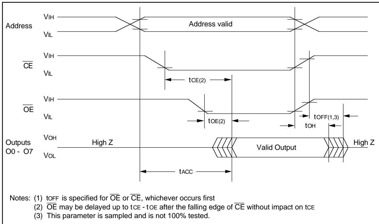
FIGURE 1-1: READ WAVEFORMS
