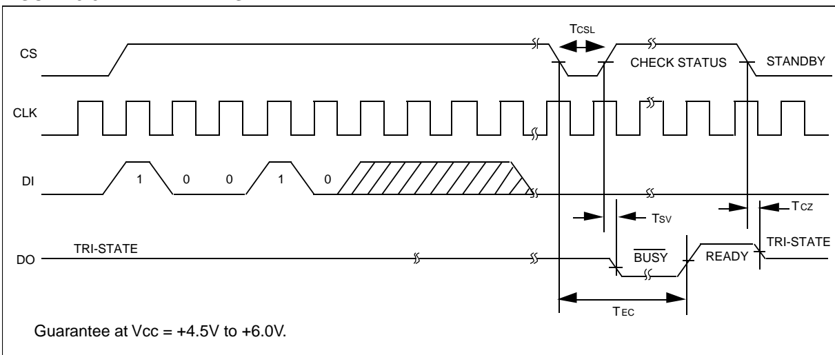
FIGURE 3-3: ERAL TIMING
