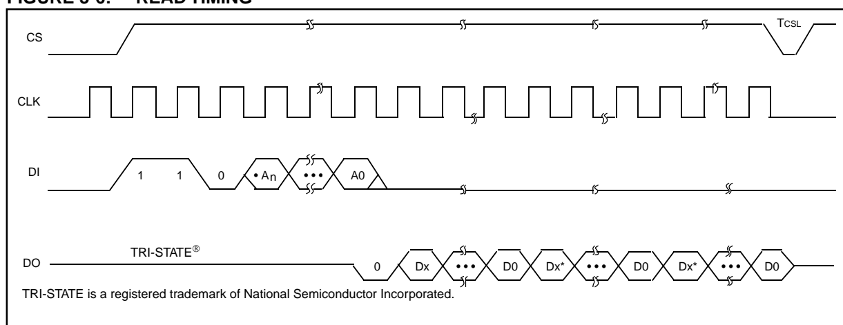
FIGURE 3-6: READ TIMING
