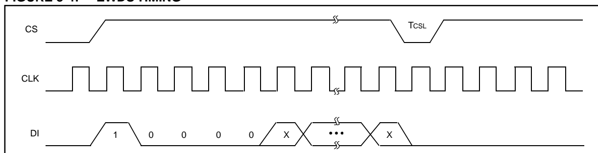
FIGURE 3-5: EWEN TIMING
