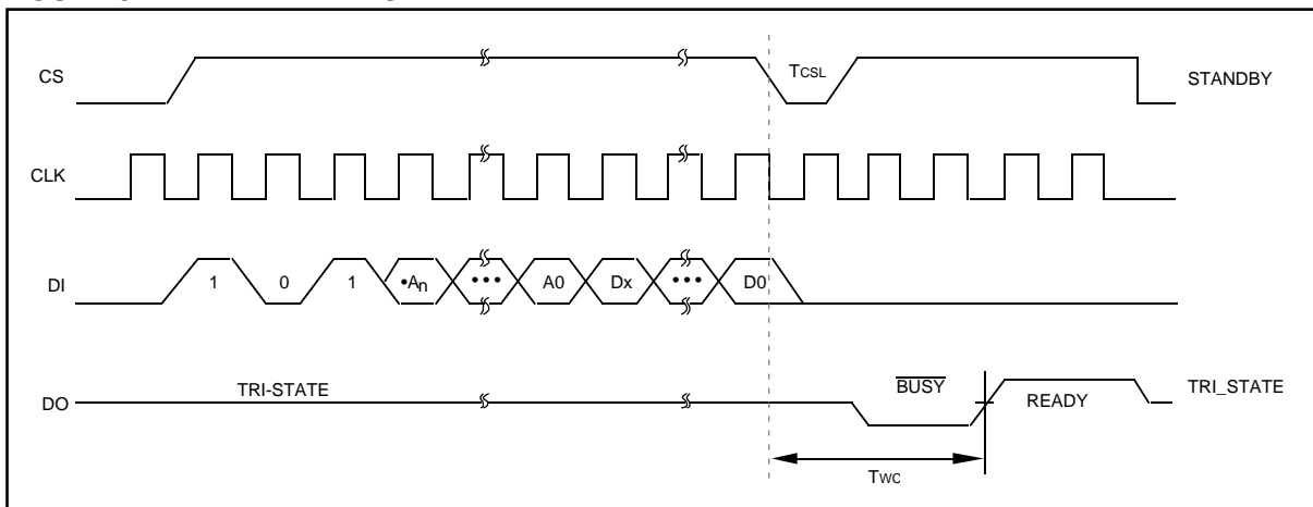
FIGURE 3-8: WRAL TIMING
