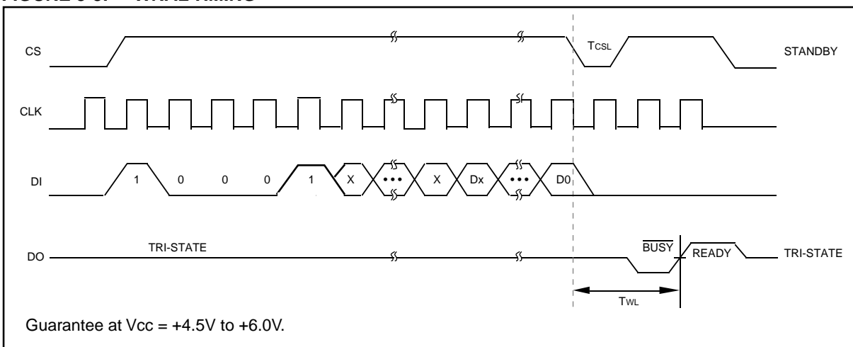
FIGURE 3-8: WRAL TIMING
