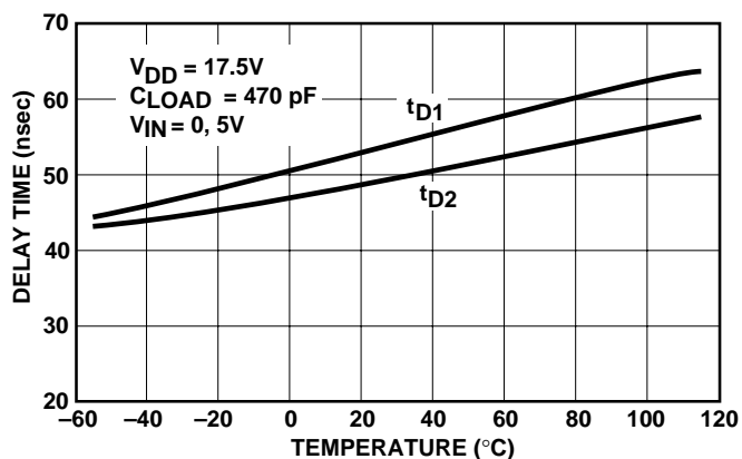
Propagation Delay Times vs. Temperature
