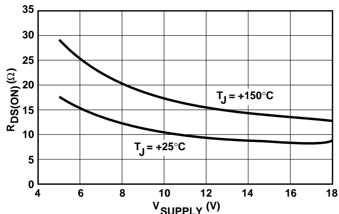
Low-State Output Resistance
