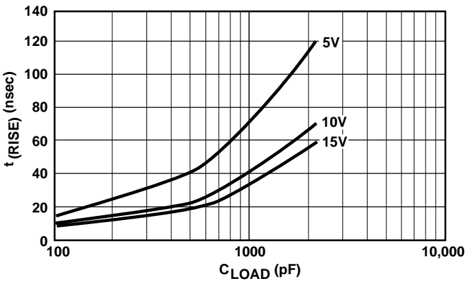
Rise Time vs. Capacitive Load
