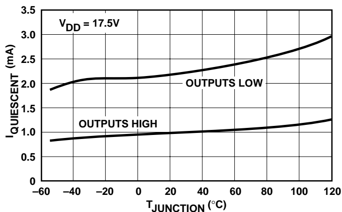
Quiescent Supply Current vs. Temperature
