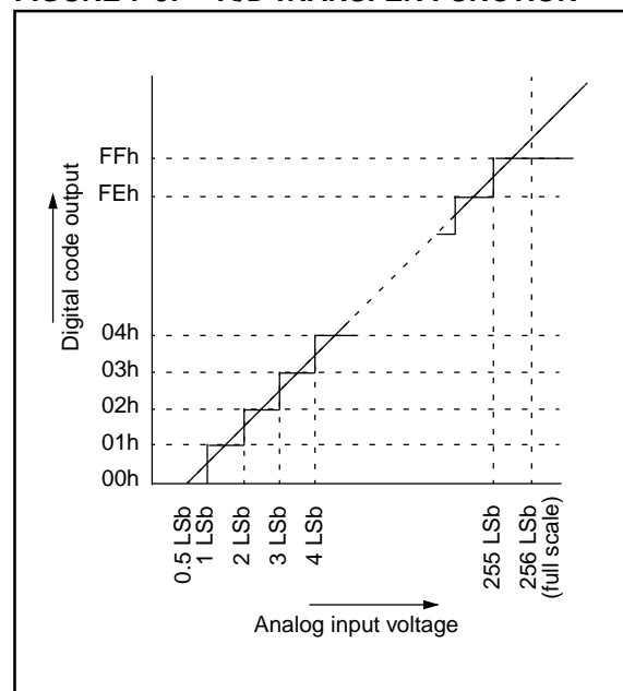
FIGURE 7-5: A/D TRANSFER FUNCTION
