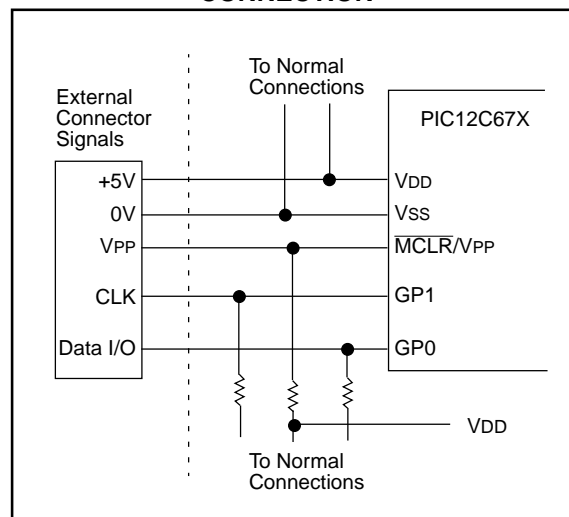
FIGURE 8-19: TYPICAL IN-CIRCUIT SERIAL PROGRAMMING CONNECTION
