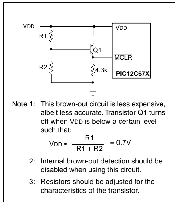
FIGURE 8-13: EXTERNAL BROWN-OUT PROTECTION CIRCUIT 2
