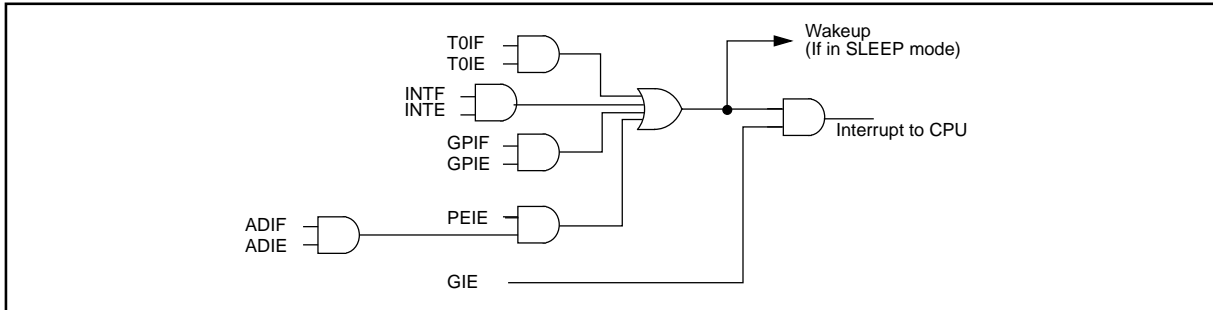
FIGURE 8-14: INTERRUPT LOGIC
