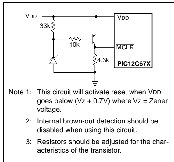
FIGURE 8-13: EXTERNAL BROWN-OUT PROTECTION CIRCUIT 2
