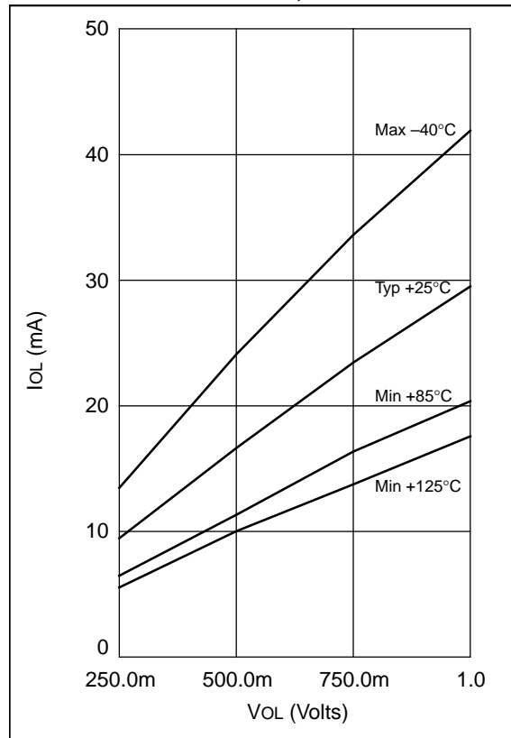
FIGURE 12-9: I_{OL} vs. V_{OL} , V_{DD} = 5.5\text{ V}
