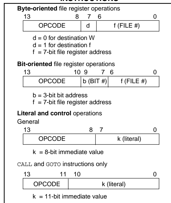
FIGURE 9-1: GENERAL FORMAT FOR INSTRUCTIONS
