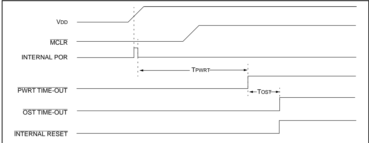
FIGURE 11-9: TIME-OUT SEQUENCE ON POWER-UP ( \overline{\text{MCLR}} NOT TIED TO V_{DD} ): CASE 2
