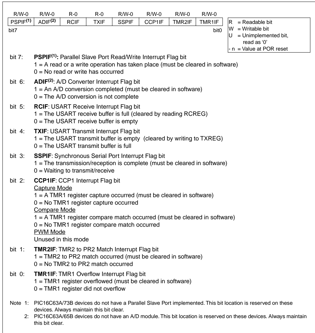
FIGURE 2-7: PIR1 REGISTER (ADDRESS 0Ch)
