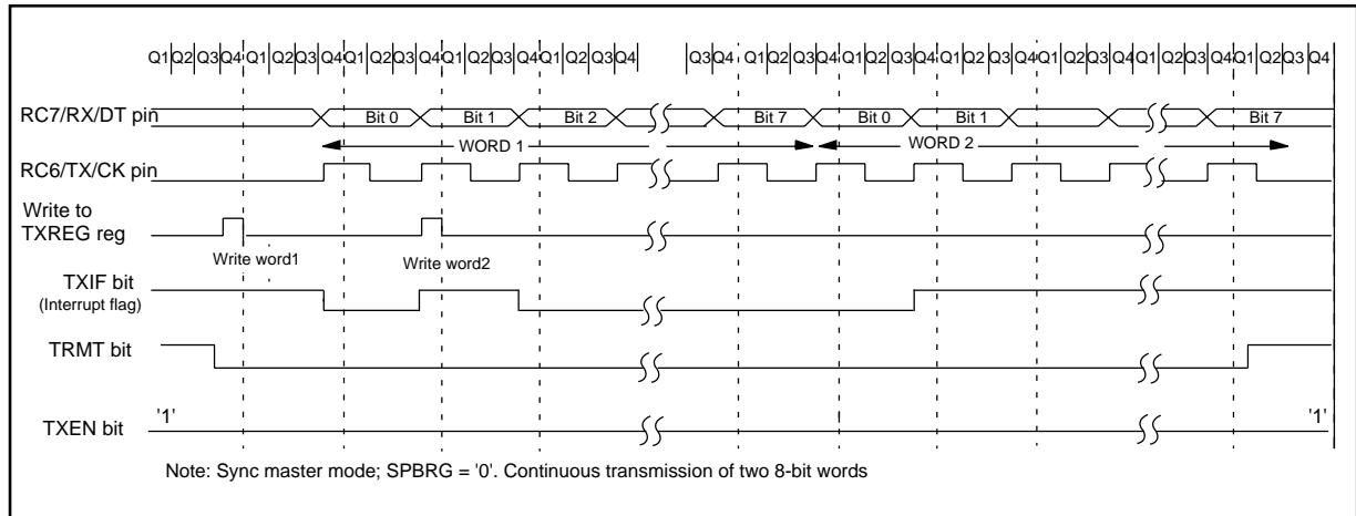
FIGURE 9-8: SYNCHRONOUS TRANSMISSION
