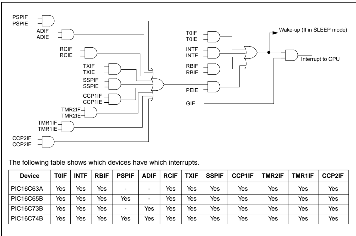
FIGURE 11-11: INTERRUPT LOGIC
