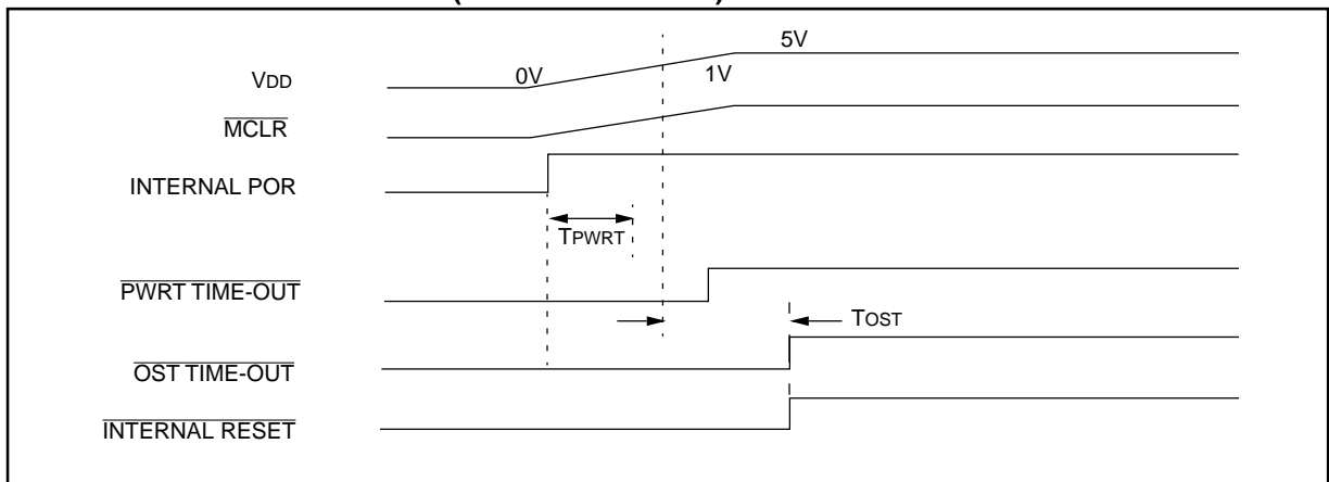
FIGURE 11-10: SLOW RISE TIME ( \overline{\text{MCLR}} TIED TO V_{DD} )
