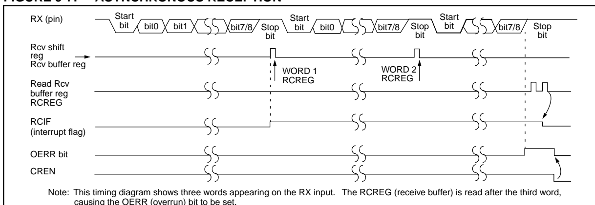
FIGURE 9-7: ASYNCHRONOUS RECEPTION
