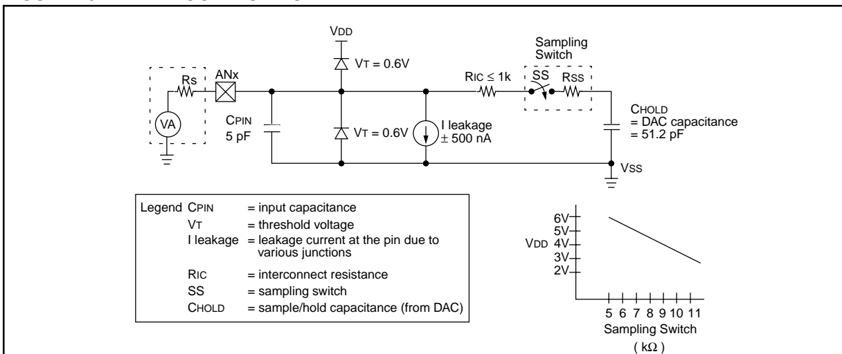
FIGURE 10-4: ANALOG INPUT MODEL
