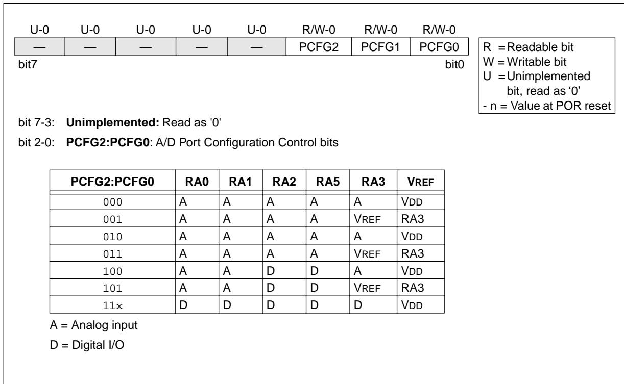
FIGURE 10-2: ADCON1 REGISTER (ADDRESS 9Fh)
