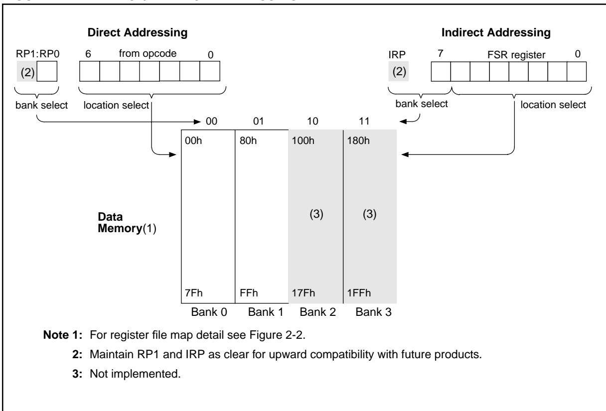
FIGURE 2-11: DIRECT/INDIRECT ADDRESSING
