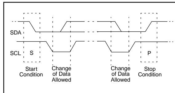
FIGURE 11-8: START AND STOP CONDITIONS
