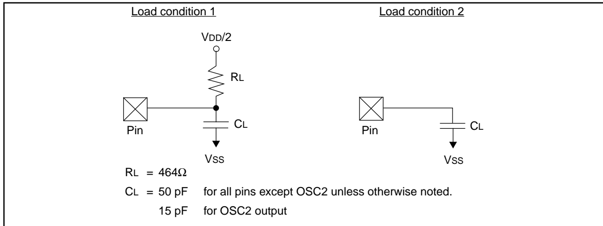
FIGURE 17-2: LOAD CONDITIONS
