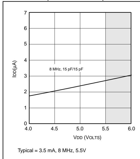
FIGURE 18-30:TYPICAL I_{DD} vs. V_{DD} (HS MODE @ 25°C)
