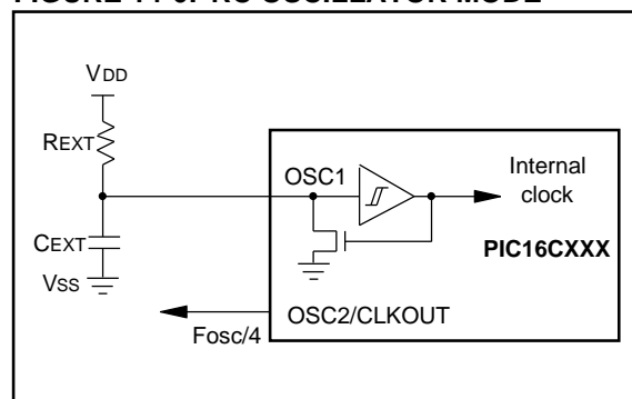
FIGURE 14-6: RC OSCILLATOR MODE
