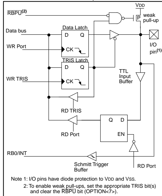
FIGURE 5-5: PORTC BLOCK DIAGRAM (PERIPHERAL OUTPUT OVERRIDE)
