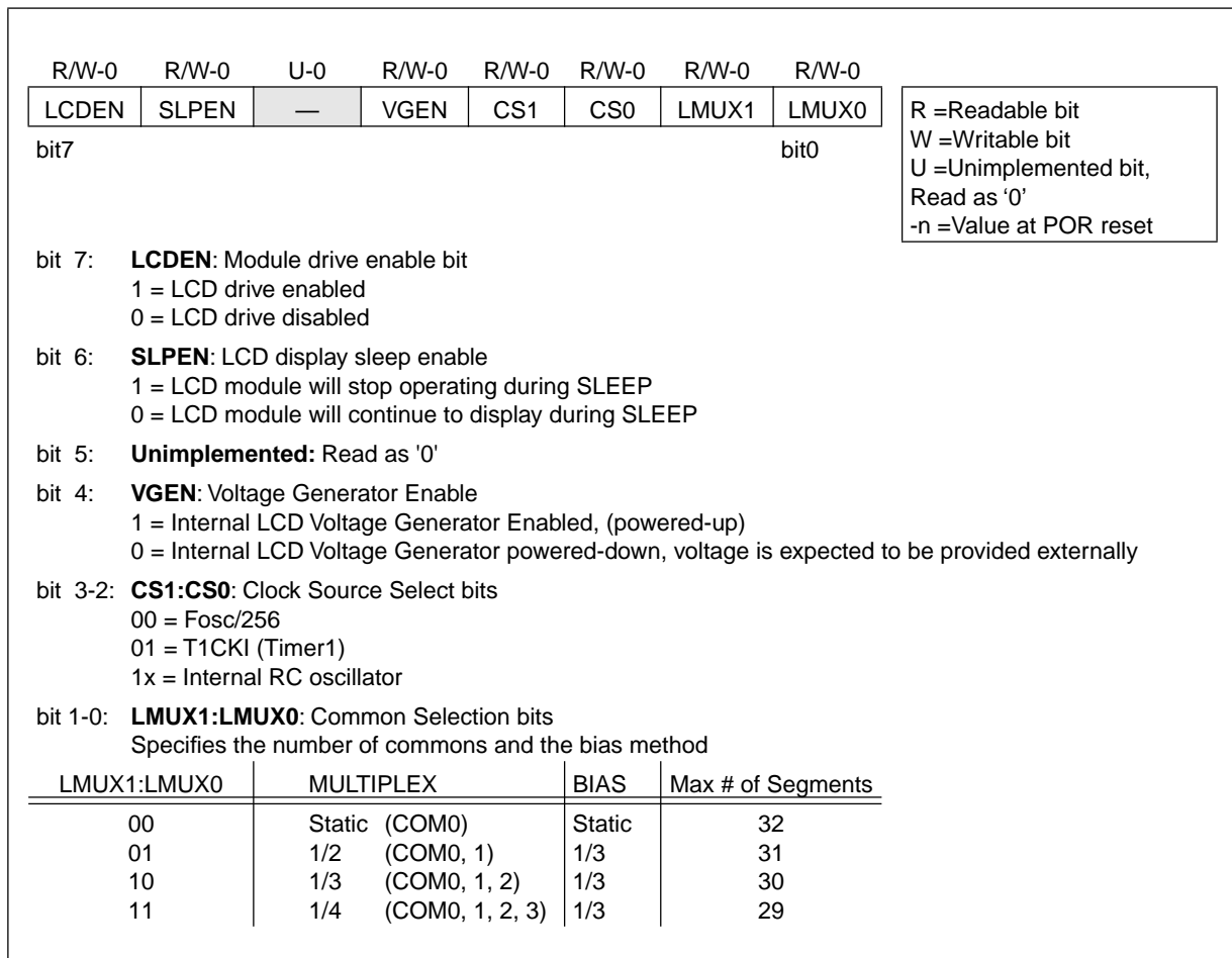
FIGURE 13-1: LCDCON REGISTER (ADDRESS 10Fh)
