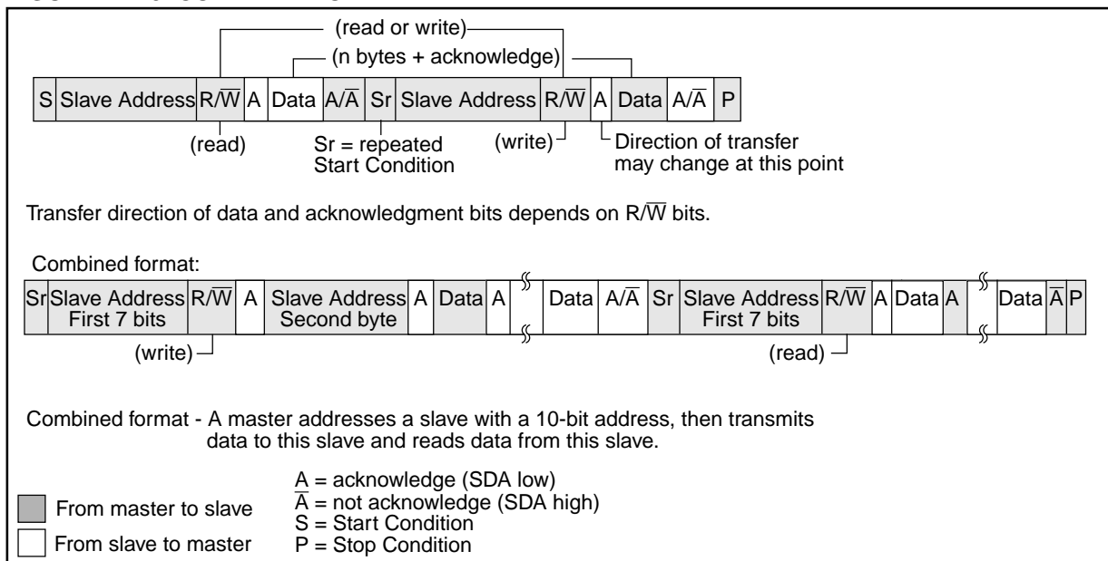
FIGURE 11-15: COMBINED FORMAT
