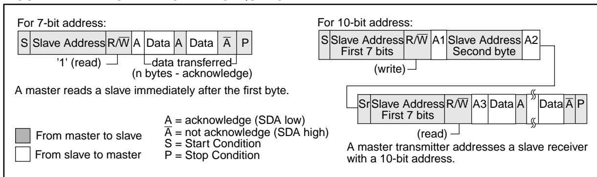
FIGURE 11-14: MASTER-RECEIVER SEQUENCE
