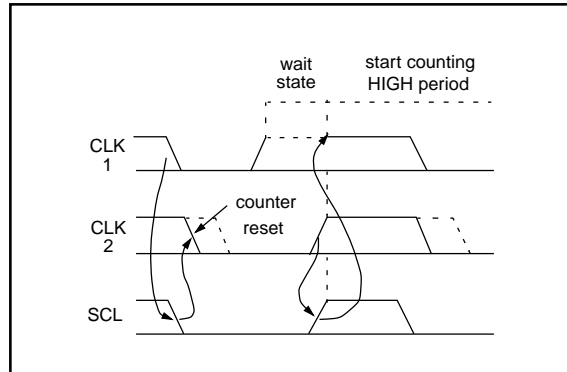
FIGURE 11-17: CLOCK SYNCHRONIZATION
