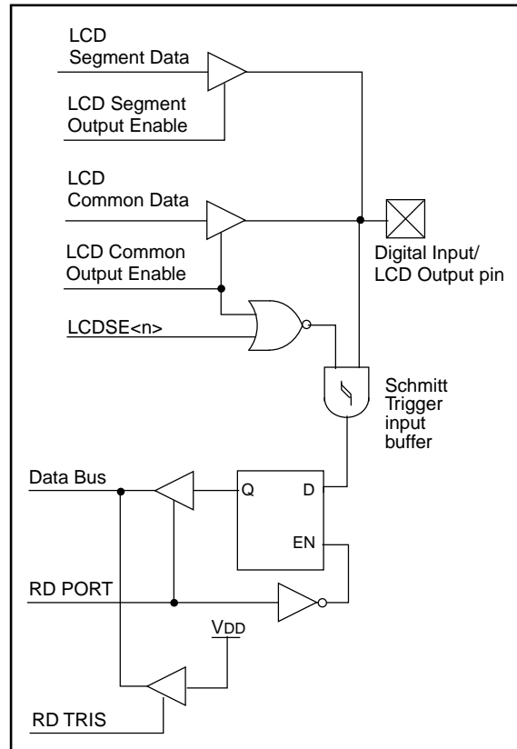
FIGURE 5-9: PORTF BLOCK DIAGRAM
