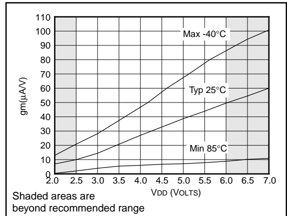
FIGURE 18-22: TRANSCONDUCTANCE(gm) OF XT OSCILLATOR vs. VDD
