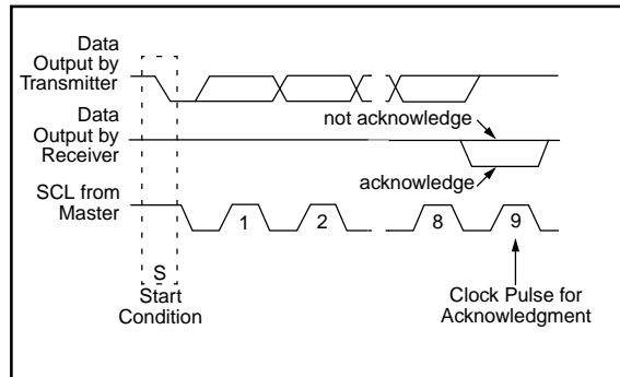
FIGURE 11-11: SLAVE-RECEIVER ACKNOWLEDGE
