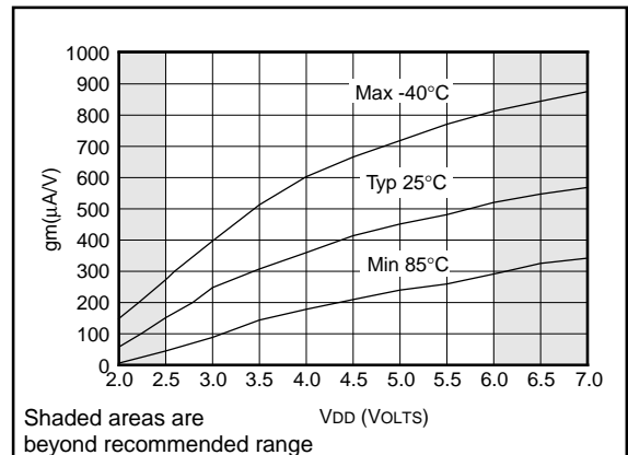
FIGURE 18-22: TRANSCONDUCTANCE(gm) OF XT OSCILLATOR vs. VDD
