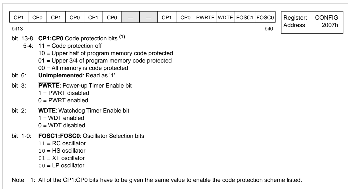
FIGURE 14-1: CONFIGURATION WORD
