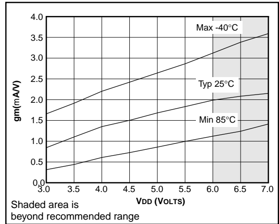
FIGURE 18-21: TRANSCONDUCTANCE(gm) OF LP OSCILLATOR vs. VDD
