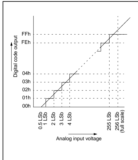
FIGURE 12-5: A/D TRANSFER FUNCTION
