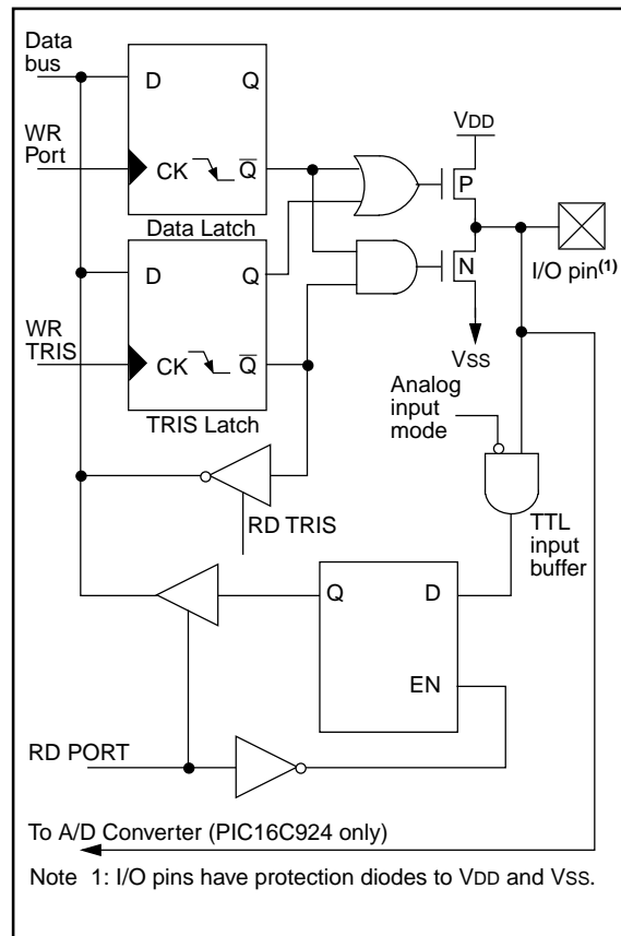
FIGURE 5-1: BLOCK DIAGRAM OF PINS RA3:RA0 AND RA5
