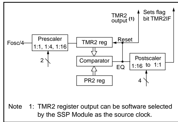
FIGURE 9-1: TIMER2 BLOCK DIAGRAM
