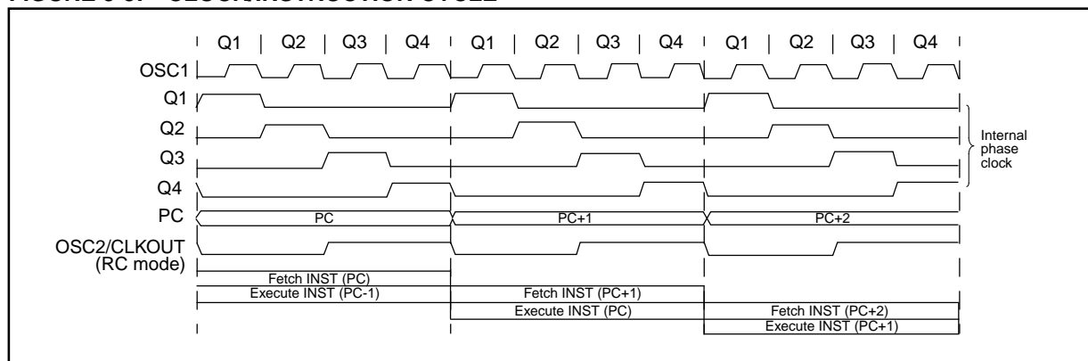
FIGURE 3-3: CLOCK/INSTRUCTION CYCLE
