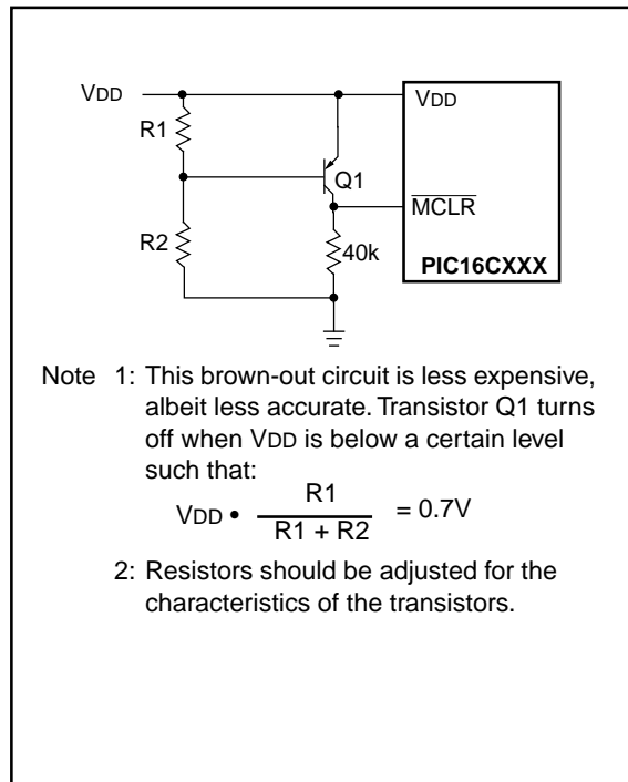
FIGURE 14-13:EXTERNAL BROWN-OUT PROTECTION CIRCUIT 2
