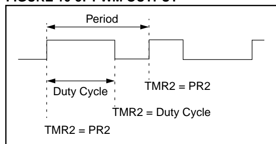
FIGURE 10-5: PWM OUTPUT
