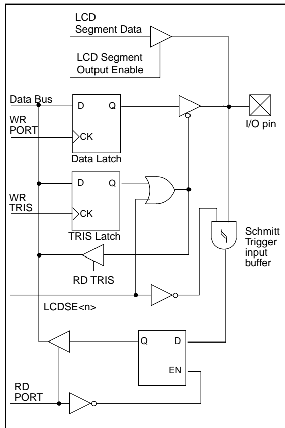
FIGURE 5-6: PORTD<4:0> BLOCK DIAGRAM
