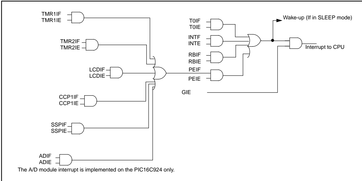
FIGURE 14-14: INTERRUPT LOGIC
