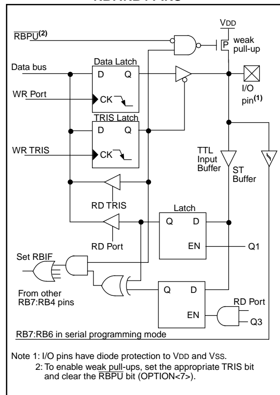
FIGURE 5-4: BLOCK DIAGRAM OF RB7:RB4 PINS
