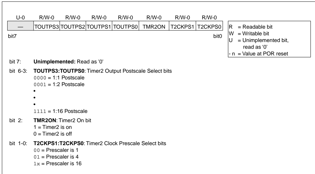
FIGURE 9-2: T2CON: TIMER2 CONTROL REGISTER (ADDRESS 12h)
