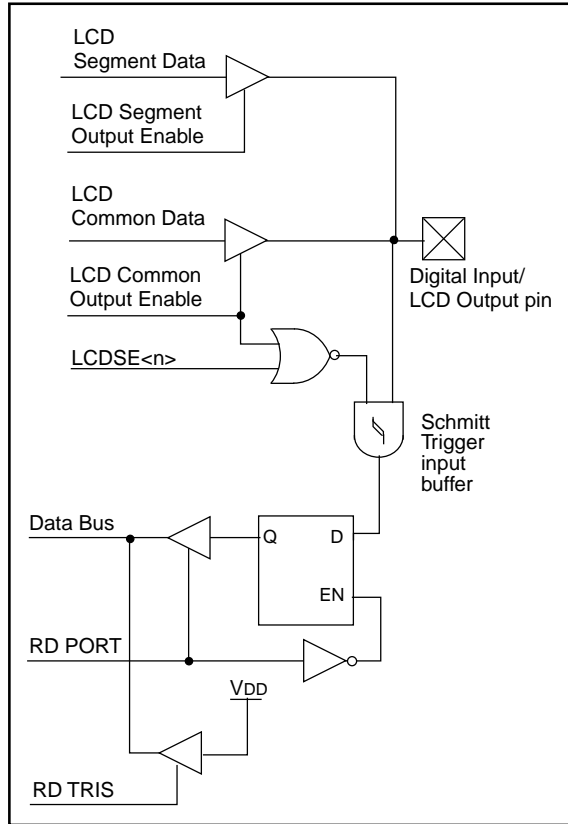
FIGURE 5-10: PORTG BLOCK DIAGRAM
