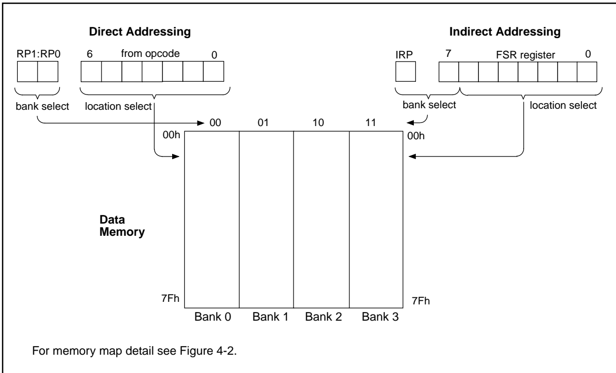
FIGURE 4-10: DIRECT/INDIRECT ADDRESSING
