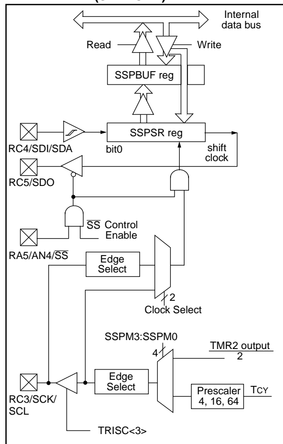
FIGURE 11-3: SSP BLOCK DIAGRAM (SPI MODE)
