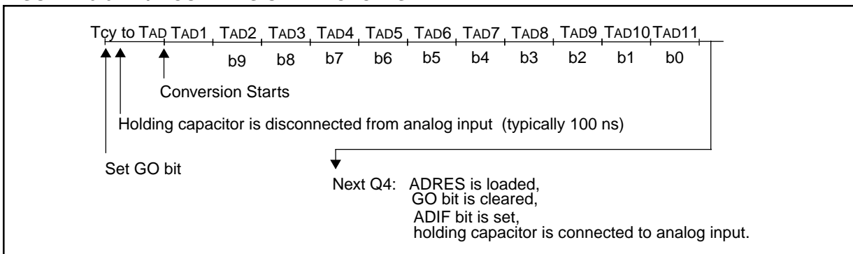
FIGURE 16-6: A/D CONVERSION TAD CYCLES
