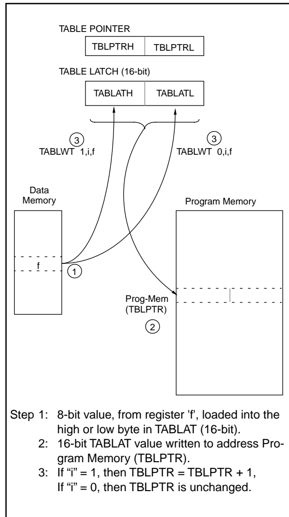
FIGURE 8-2: TABLWT INSTRUCTION OPERATION
