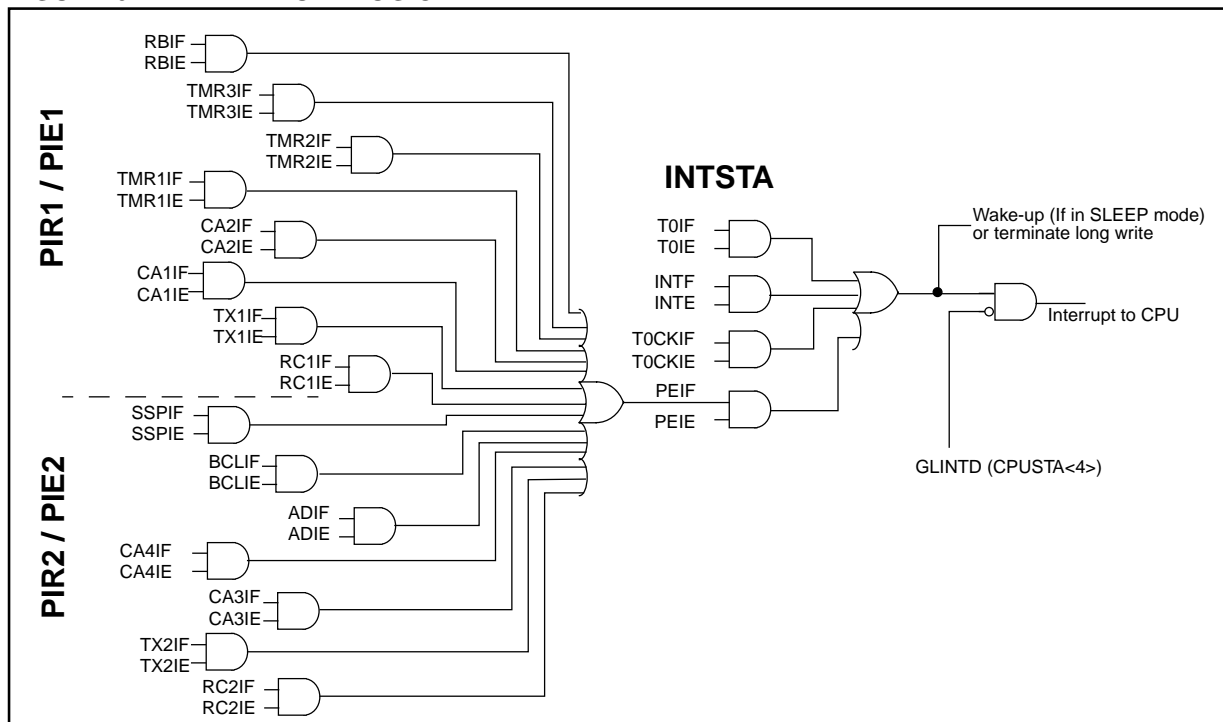
FIGURE 6-1: INTERRUPT LOGIC
