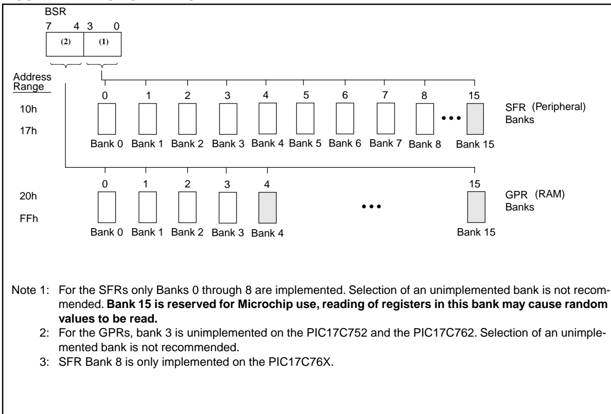
FIGURE 7-12: BSR OPERATION
