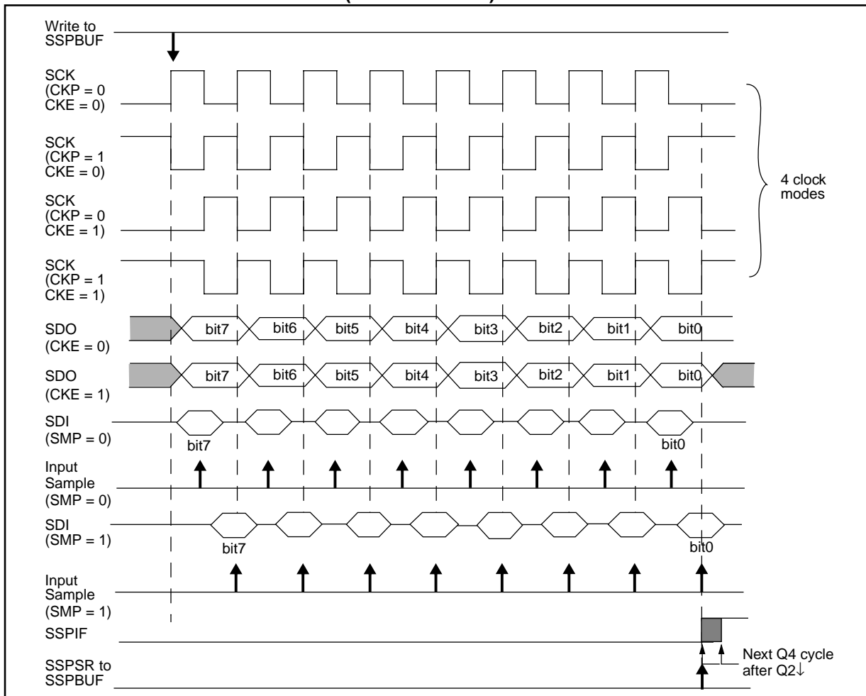
FIGURE 15-9: SPI MODE WAVEFORM (MASTER MODE)
