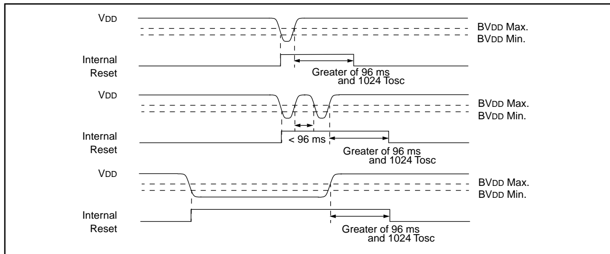
FIGURE 5-10: BROWN-OUT SITUATIONS
