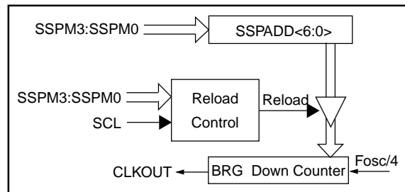
FIGURE 15-21: BAUD RATE GENERATOR BLOCK DIAGRAM
