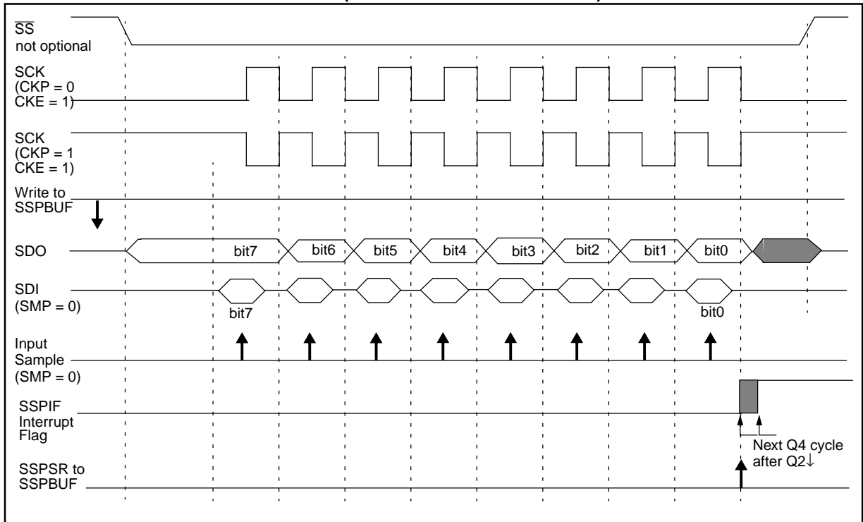
FIGURE 15-12: SPI MODE WAVEFORM (SLAVE MODE WITH CKE = 1)
