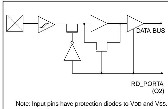
FIGURE 10-2: RA2 BLOCK DIAGRAM
