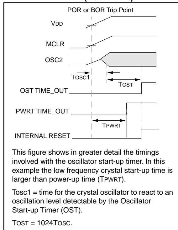
FIGURE 5-4: OSCILLATOR START-UP TIME (LOW FREQ)
