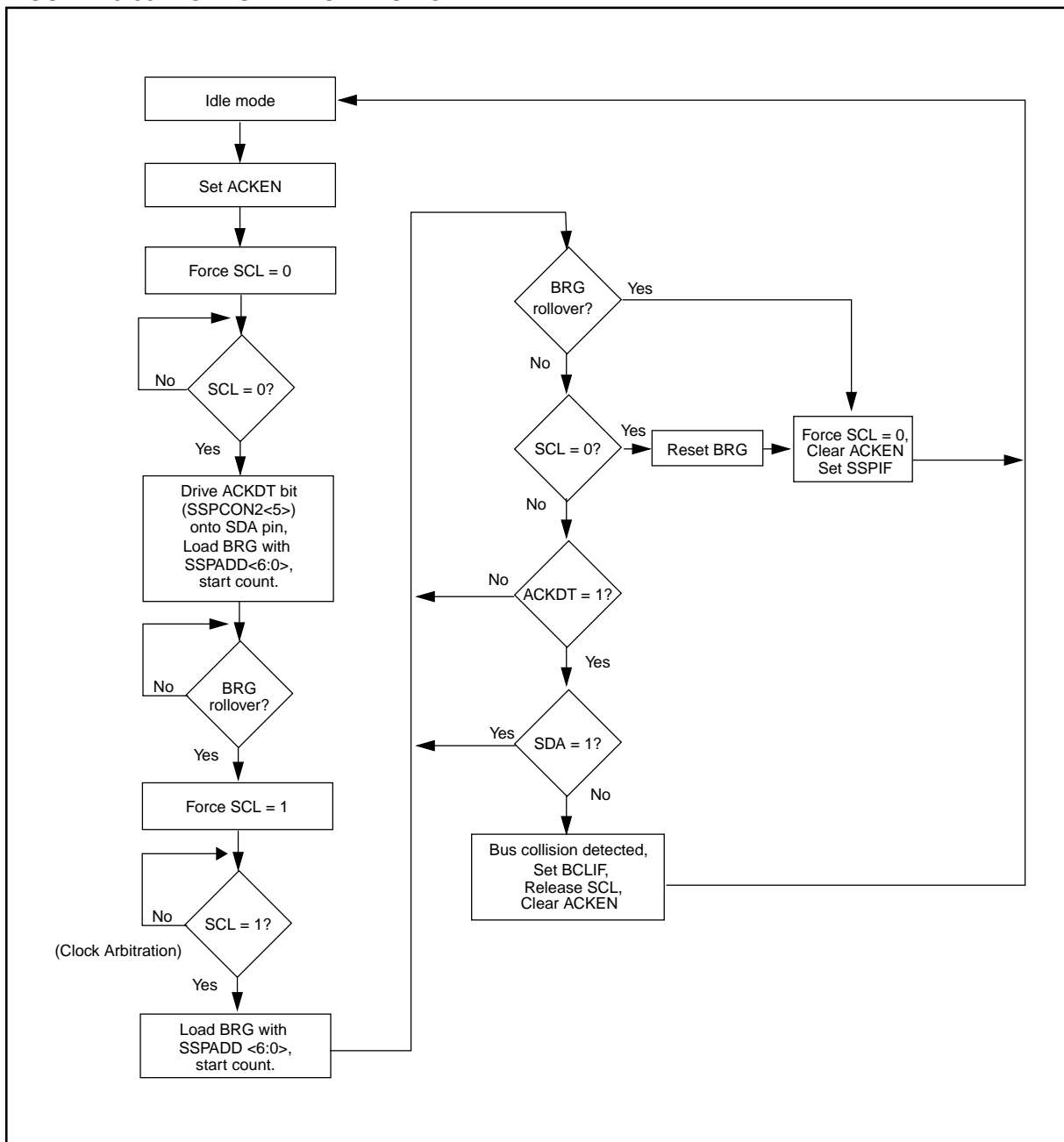
FIGURE 15-33: ACKNOWLEDGE FLOWCHART
