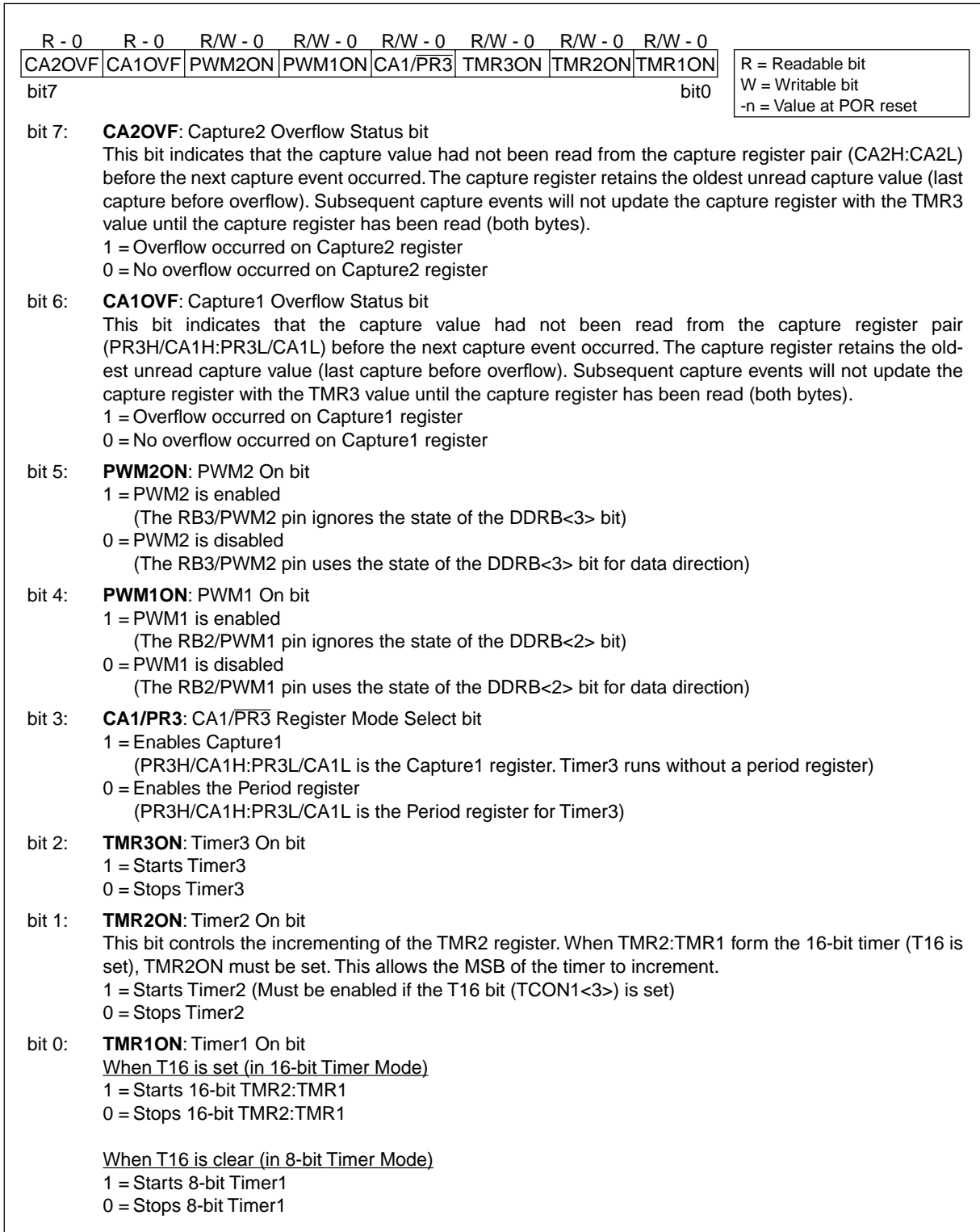
FIGURE 13-2: TCON2 REGISTER (ADDRESS: 17h, BANK 3)
