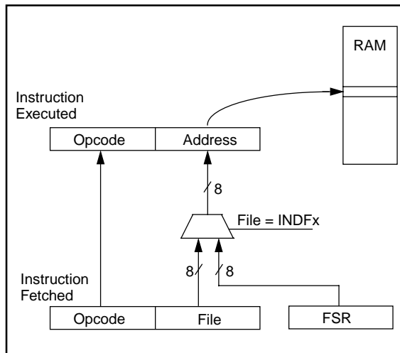
FIGURE 7-9: INDIRECT ADDRESSING
