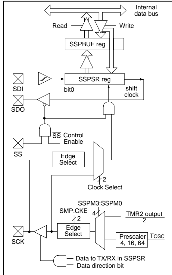
FIGURE 15-7: MSSP BLOCK DIAGRAM (SPI MODE)
