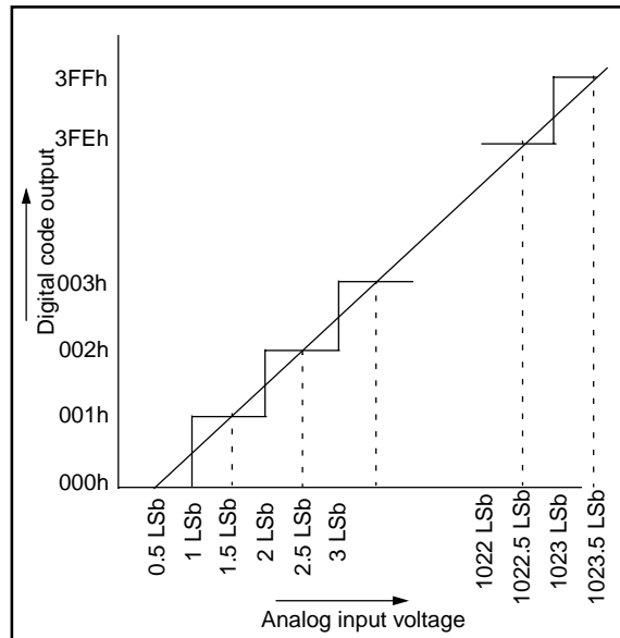
FIGURE 16-9: A/D TRANSFER FUNCTION
