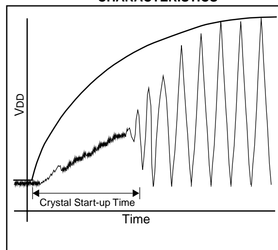
FIGURE 4-1: OSCILLATOR / RESONATOR START-UP CHARACTERISTICS
