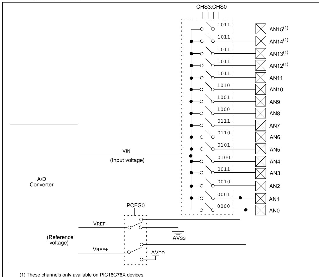
FIGURE 16-3: A/D BLOCK DIAGRAM
