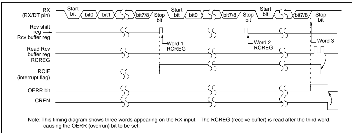
FIGURE 14-9: ASYNCHRONOUS RECEPTION
