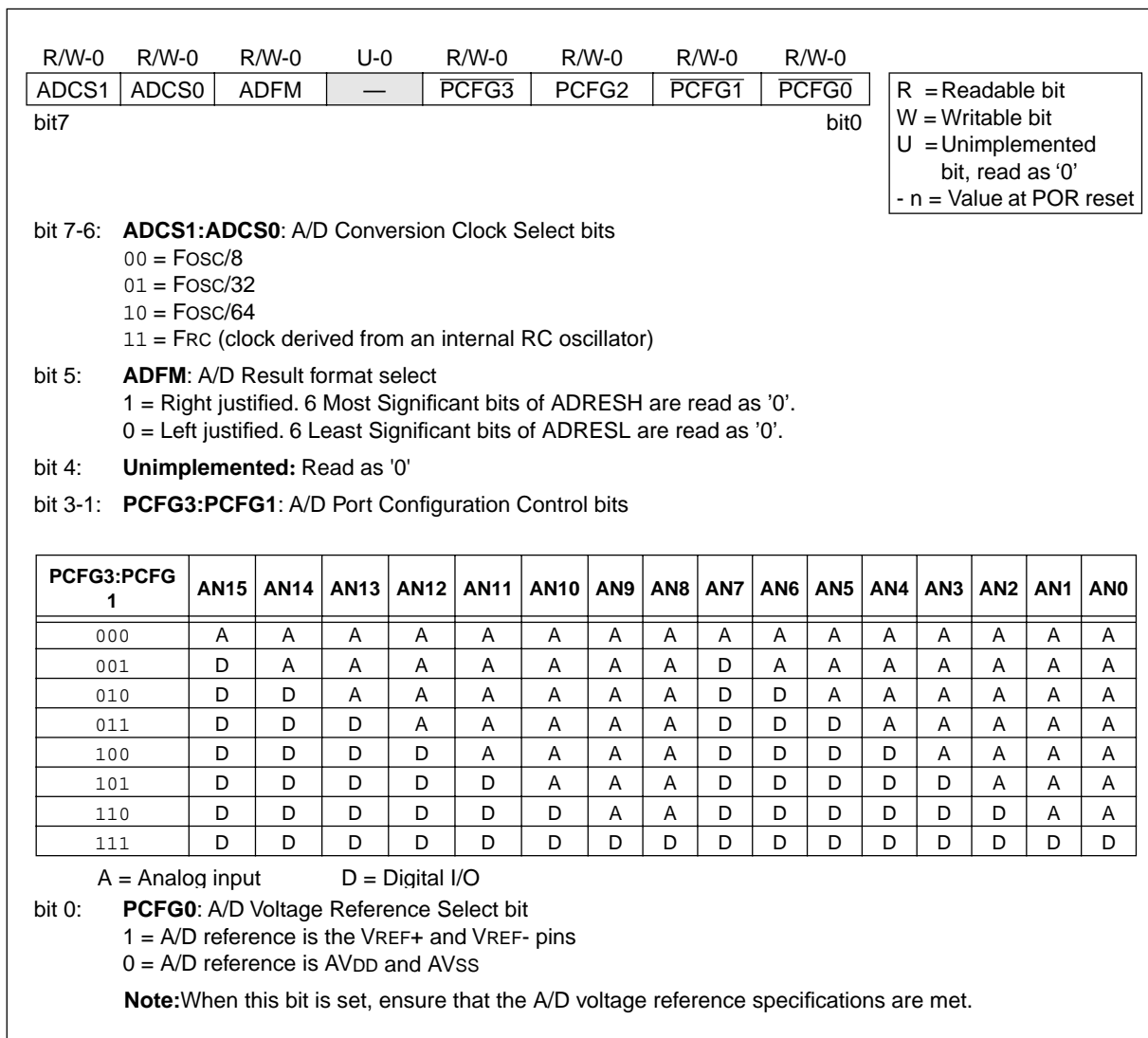
FIGURE 16-2: ADCON1 REGISTER (ADDRESS 15h, BANK 5)
