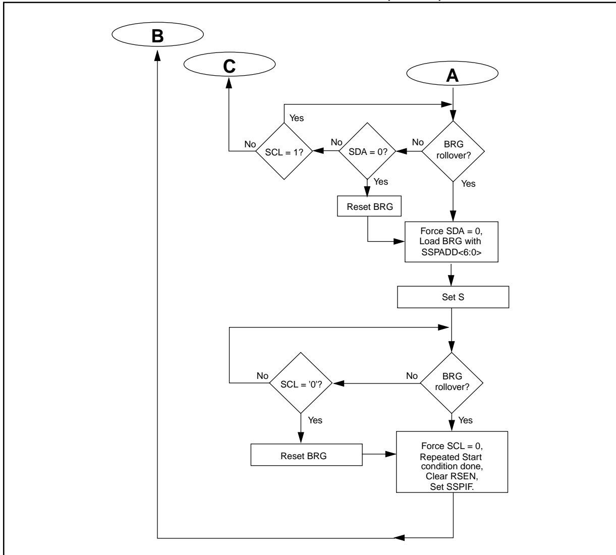
FIGURE 15-27: REPEATED START CONDITION FLOWCHART (PAGE 2)
