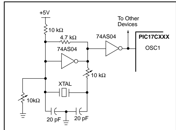
FIGURE 4-5: EXTERNAL PARALLEL RESONANT CRYSTAL OSCILLATOR CIRCUIT
