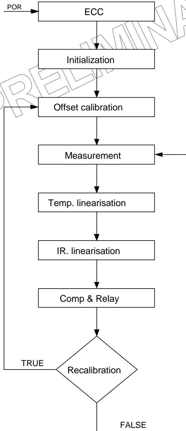
Main state machine control flow
