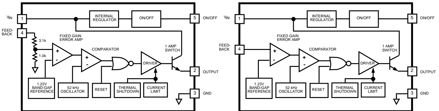
Fixed Regulator
