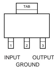
MIC2920A-x.xBS (SOT-223)
