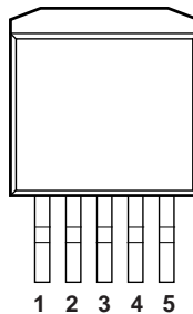
MIC29201/29202BU (TO-263-5)
