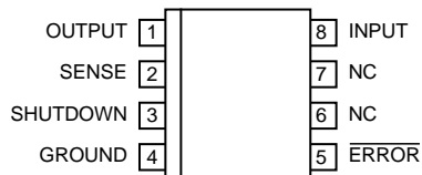
MIC29201-3.3BM (SO-8)
