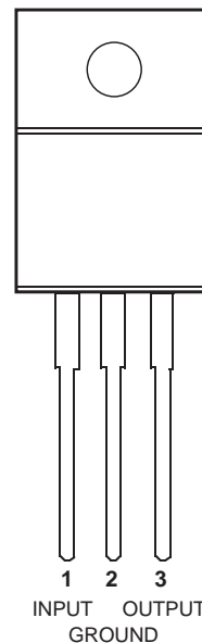
MIC2920A-xxBT (TO-220)
