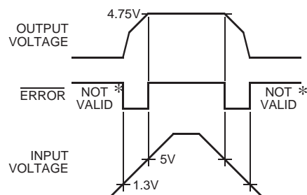
Figure 1. \overline{\text{ERROR}} Output Timing
