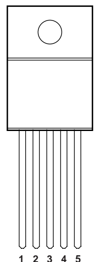
MIC29201/29202BT (TO-220-5)
