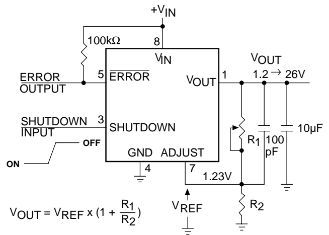
Figure 3. MIC29202/29204 Adjustable Regulator. Pinout is for MIC29204.
