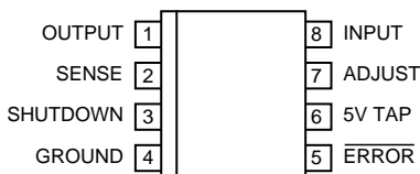
MIC29204BM (SO-8)
