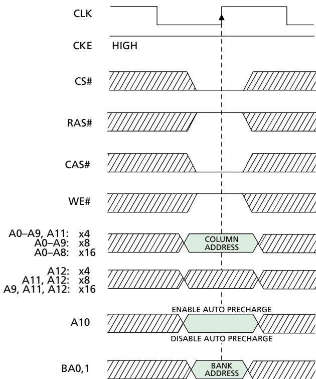
Figure 5 READ Command
