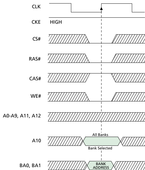
Figure 20 PRECHARGE Command
