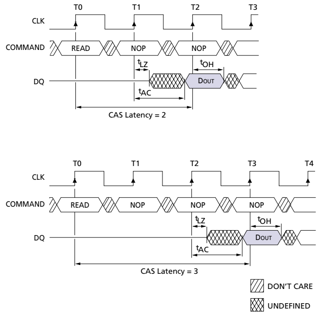
Figure 6 CAS Latency
