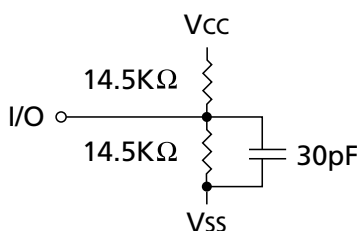
Figure 11 Output Load Circuit
