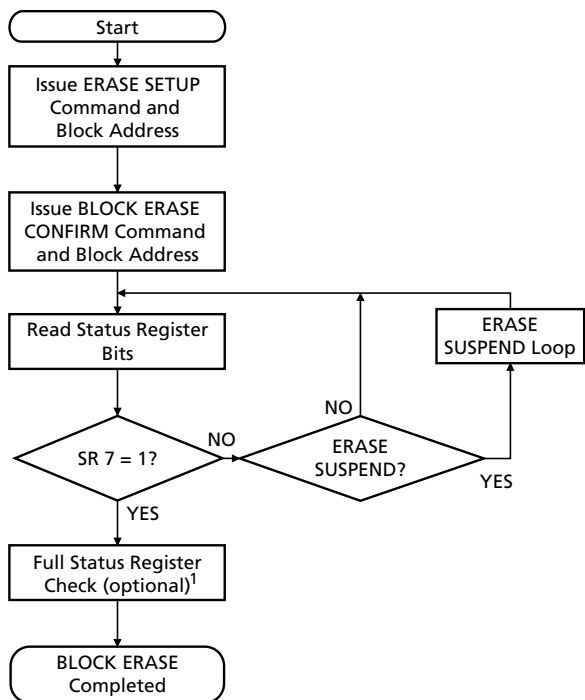
Figure 6 BLOCK ERASE Flowchart
