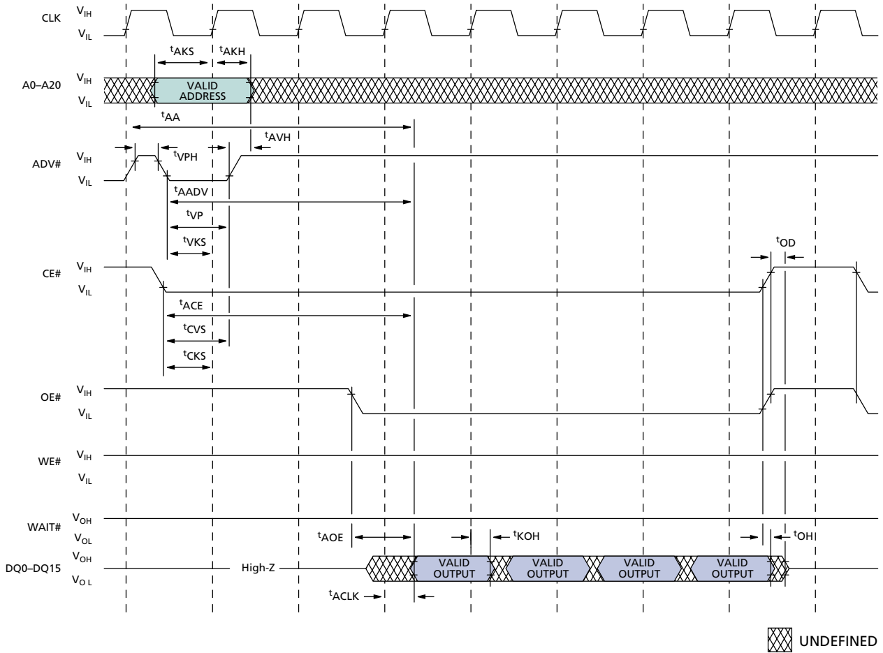
READ TIMING PARAMETERS MT28F322D20 (V CC = 1.80V–2.25V)
