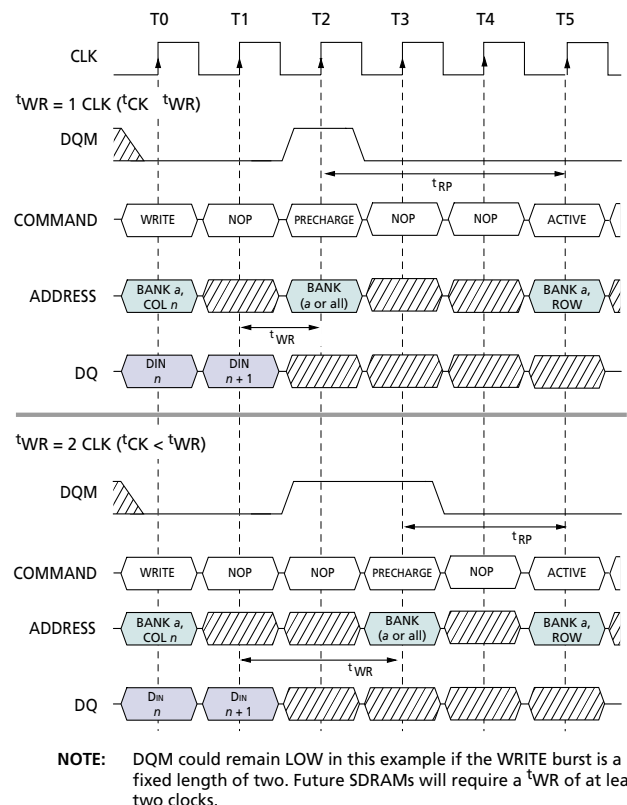
Figure 18 WRITE to PRECHARGE
