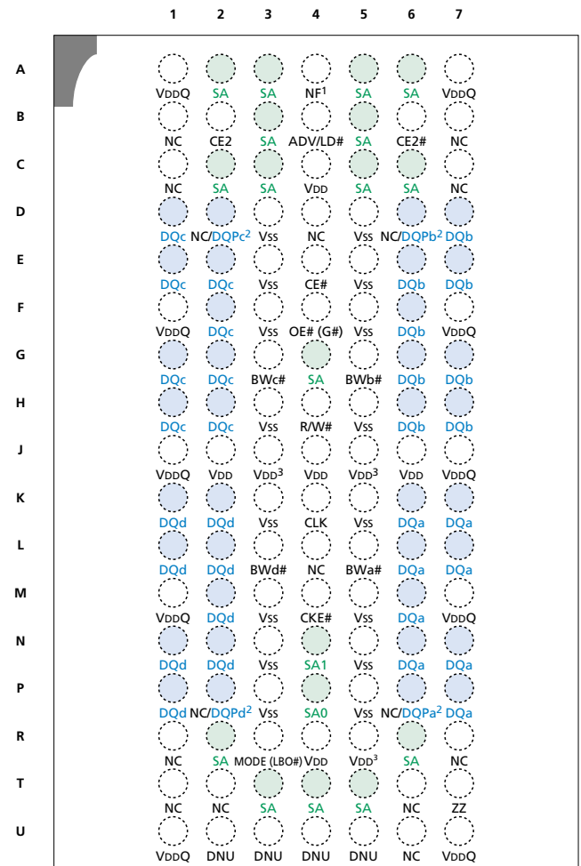
TOP VIEW
