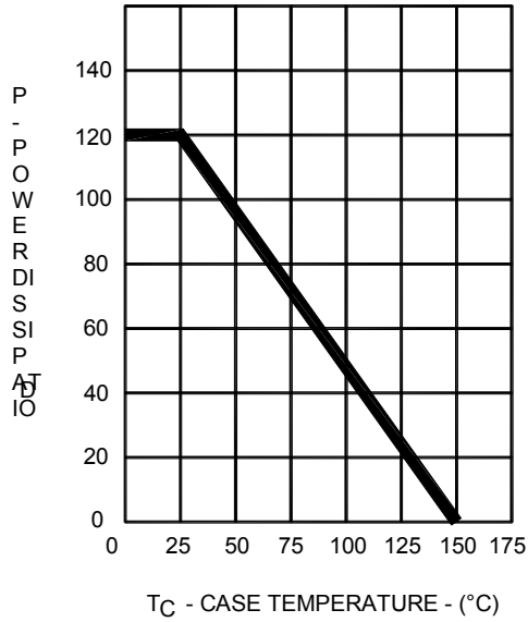
Figure 1. Power Derating
