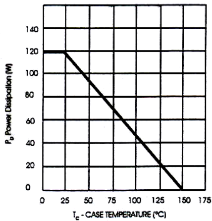
Figure 1, Power Derating
