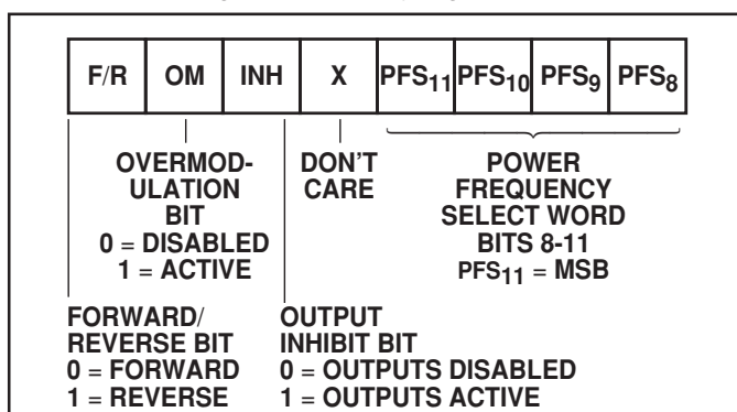
Fig. 12 Temporary register R1
