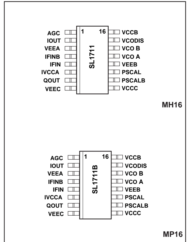
Fig. 1 Pin allocation
