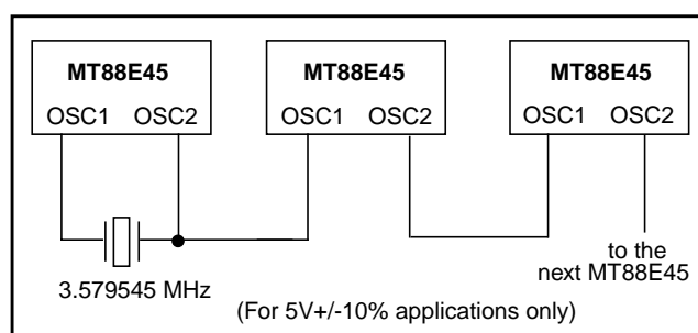
Figure 6 - Common Crystal Connection
