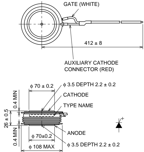
OUTLINE DRAWING
