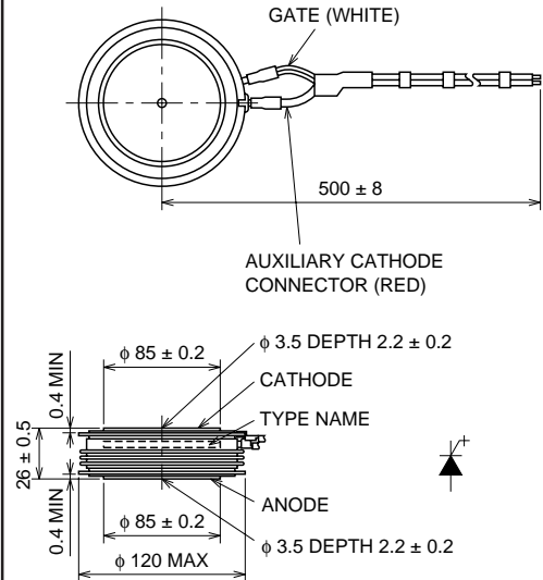
OUTLINE DRAWING
