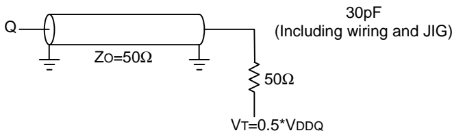
Fig.1 Output load
