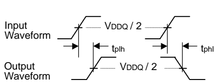
Fig.2 Tdly measurement
