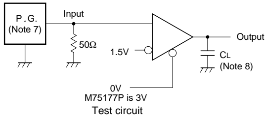
Receiver propagation delay time
