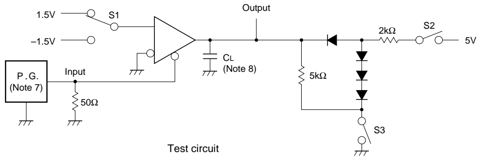
Receiver propagation delay time
