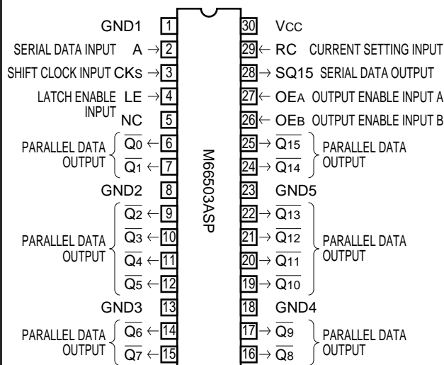
Outline 30P4B
