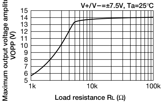
■ Example of maximum output voltage amplitude relative to load characteristics
