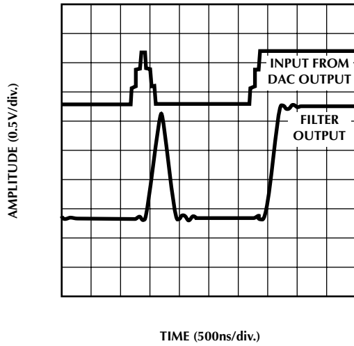
Figure 25. Transient Response
