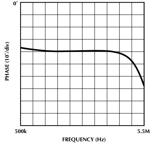
Figure 17. Deviation from Linear Phase
