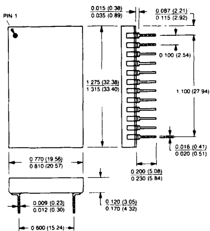
PACKAGE A
