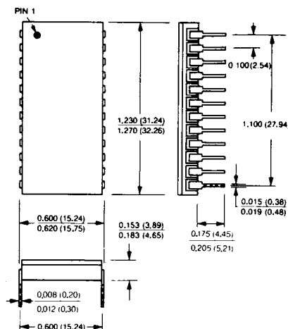
PACKAGE B
