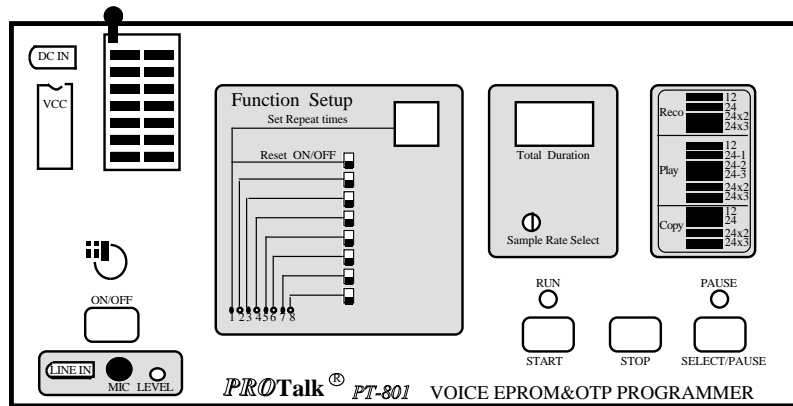
Top Panel
