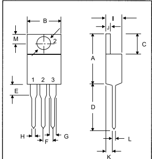
TO-220AB
