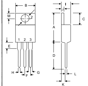
TO-220AB
