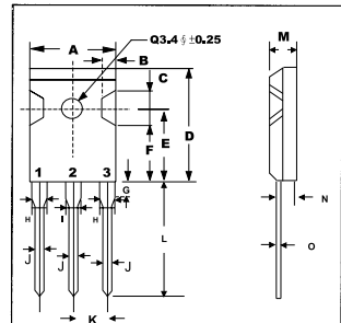
TO-247 (3P)
