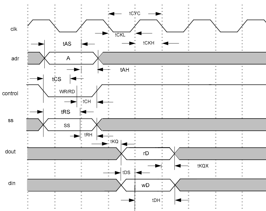
AC Timing
