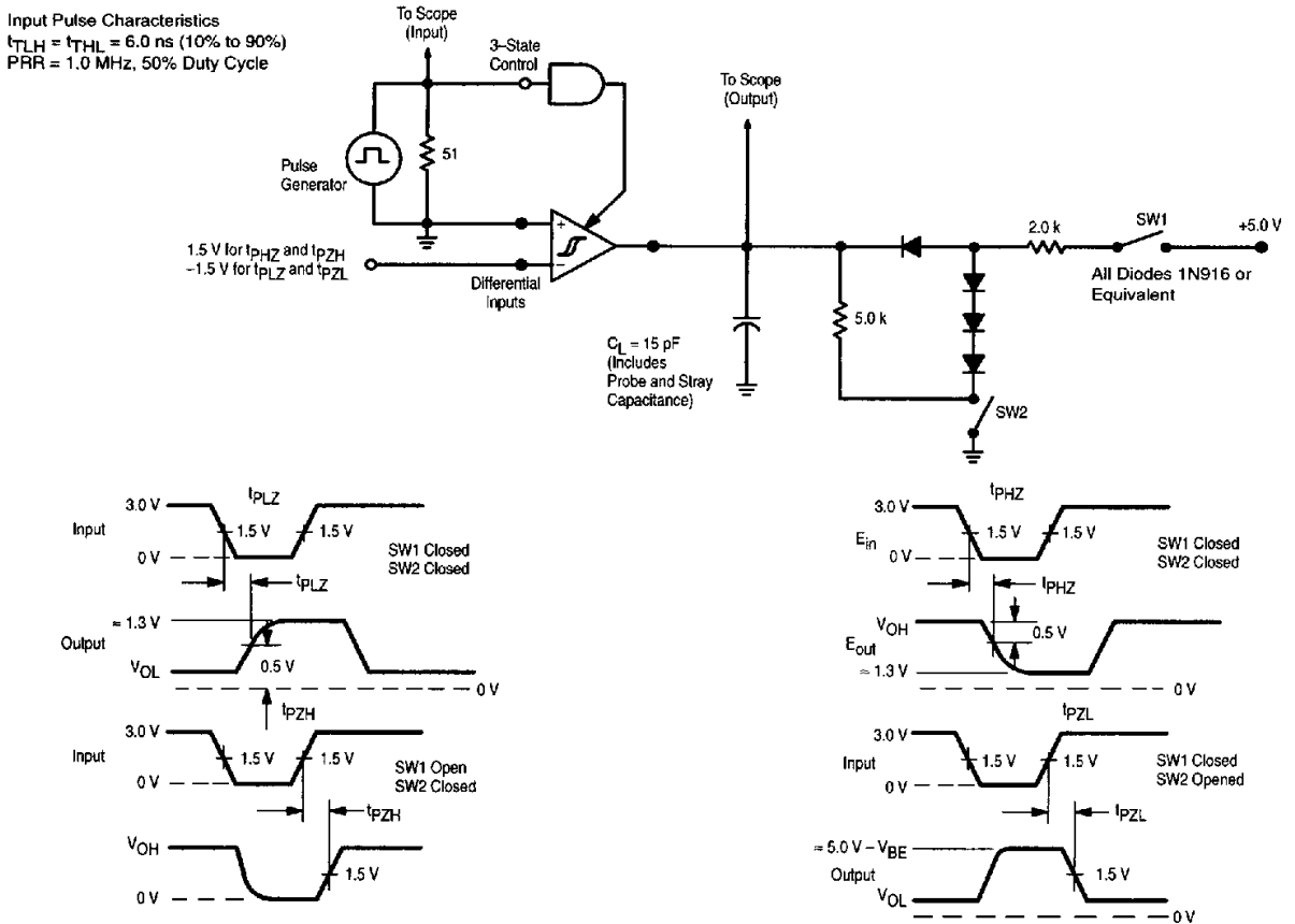
Figure 2. Propagation Delay Three-State Control Input to Output
