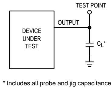
Figure 2. Test Circuit
