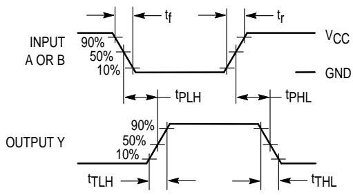
Figure 1. Switching Waveforms
