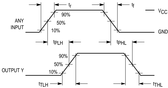
Figure 1. Switching Waveforms
