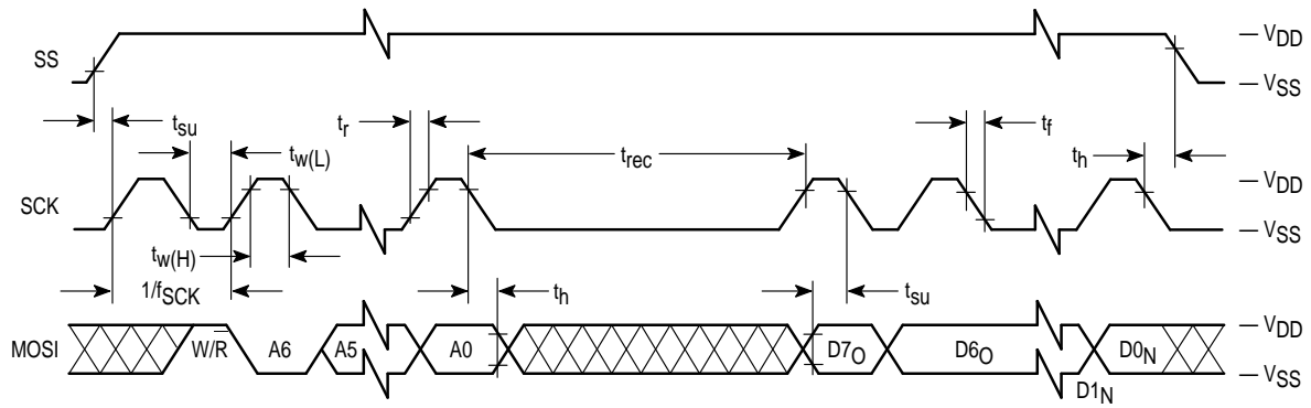
Figure 1. Write Cycle
