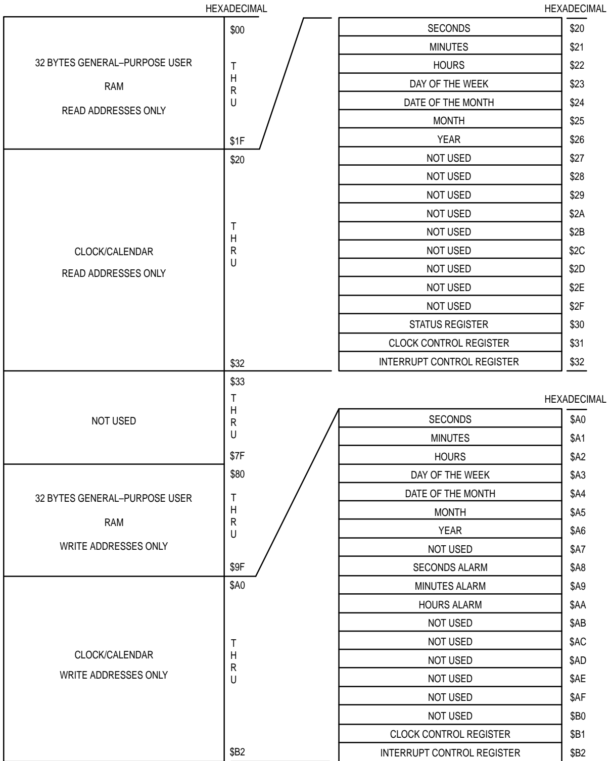
Figure 5. Address Map
