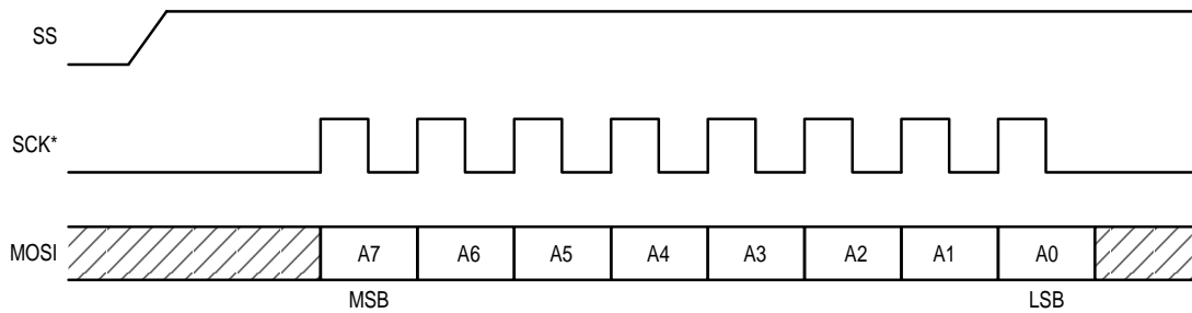
Figure 14. Address Byte Transfer Waveforms
