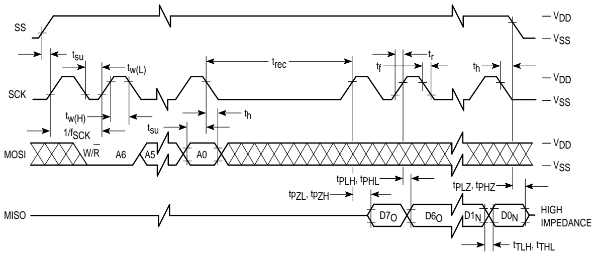
Figure 2. Read Cycle
