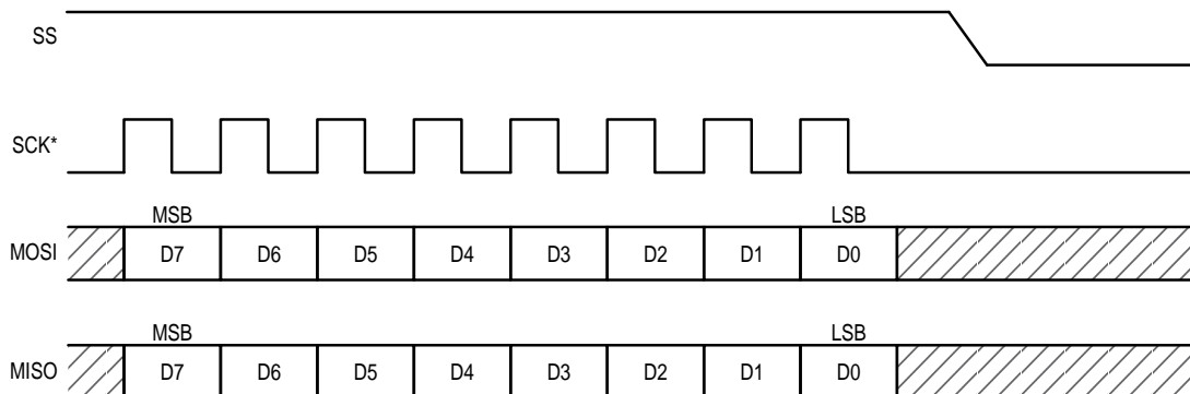
Figure 15. Read/Write Data Transfer Waveforms
