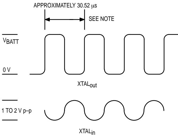
Figure 23. XTAL Waveforms
