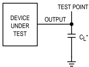
Figure 3. Test Circuit
