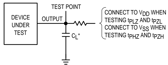
Figure 4. Test Circuit
