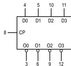
LOGIC SYMBOL
