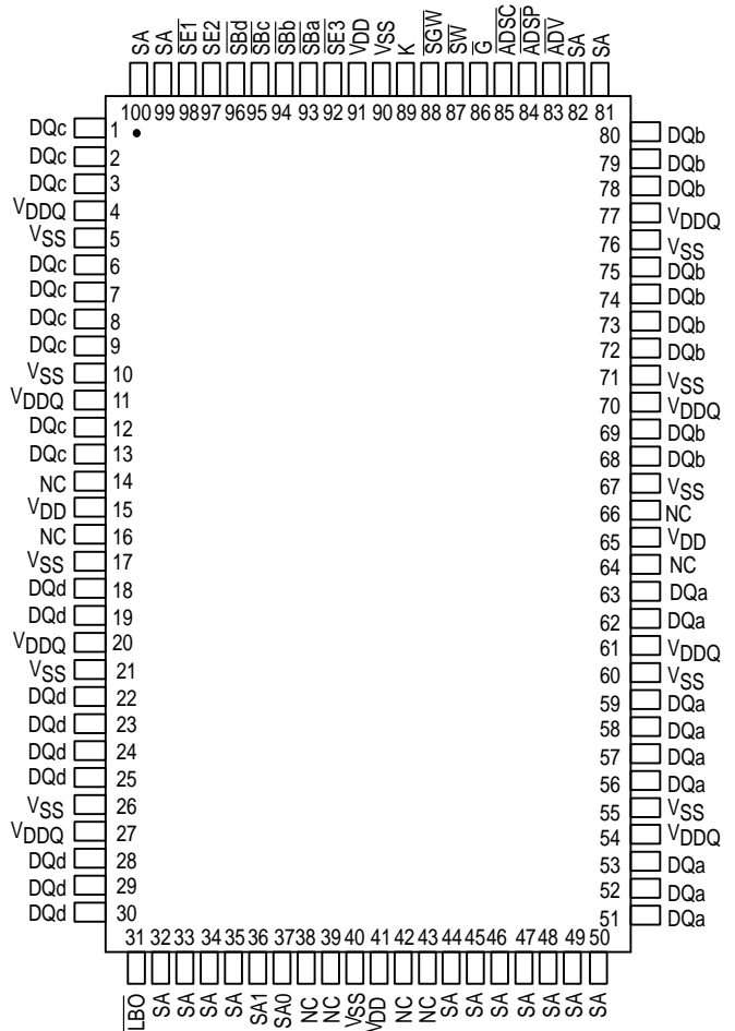
TOP VIEW 100 PIN TQFP
