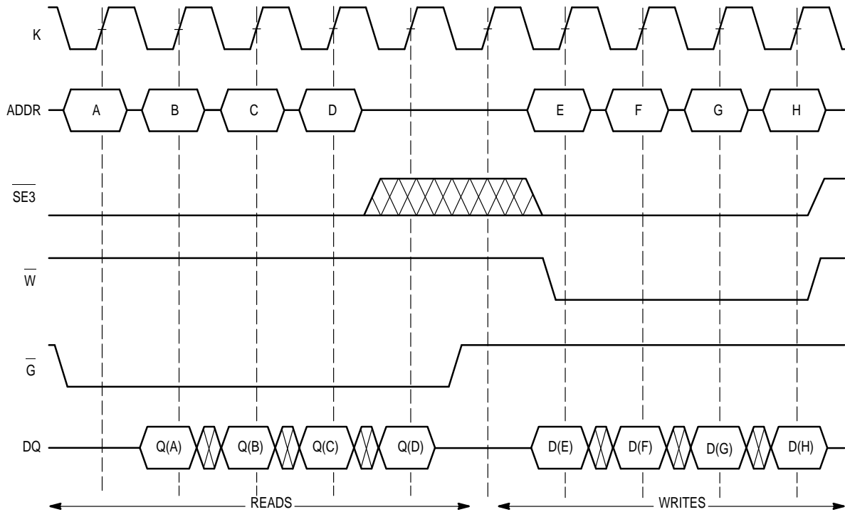
Figure 6. Example Configuration as Non-Burst Synchronous SRAM
