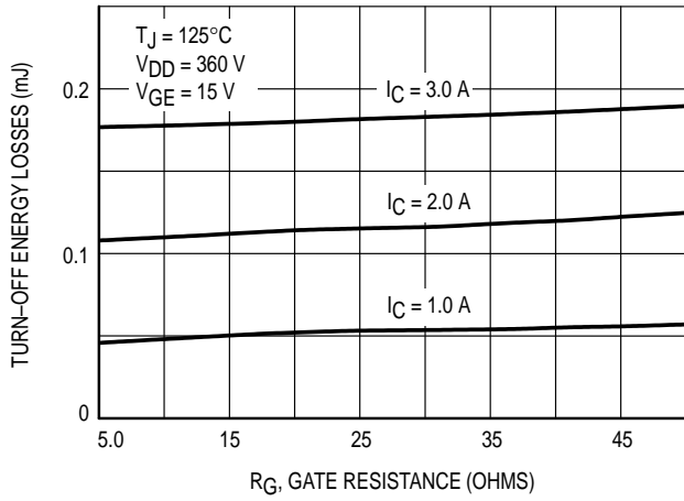
Figure 7. Turn-Off Losses versus Gate Resistance
