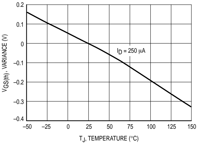
Figure 9. Threshold Voltage
