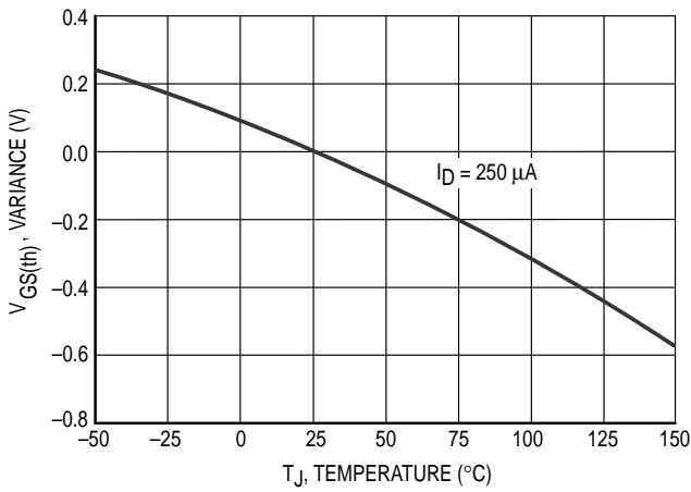
Figure 9. Threshold Voltage
